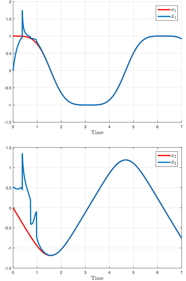
Fig. 1. Nonlinear Luenberger observer for system (15) : dynamics (16) and transformations (17) (with d_\lambda(t) = \frac{1}{\lambda} and a_\lambda(t) = \frac{1}{\lambda^2} ) for \lambda_1 = 5, \lambda_2 = 6, \lambda_3 = 7 . The transformation is inverted by first linearly combining the T_{\lambda_i} - \xi_{\lambda_i} to make x_1 disappear (because the d_{\lambda_i} are all nonzero), and then searching numerically the common roots of the obtained two polynomials of order 3 in x_2 .
