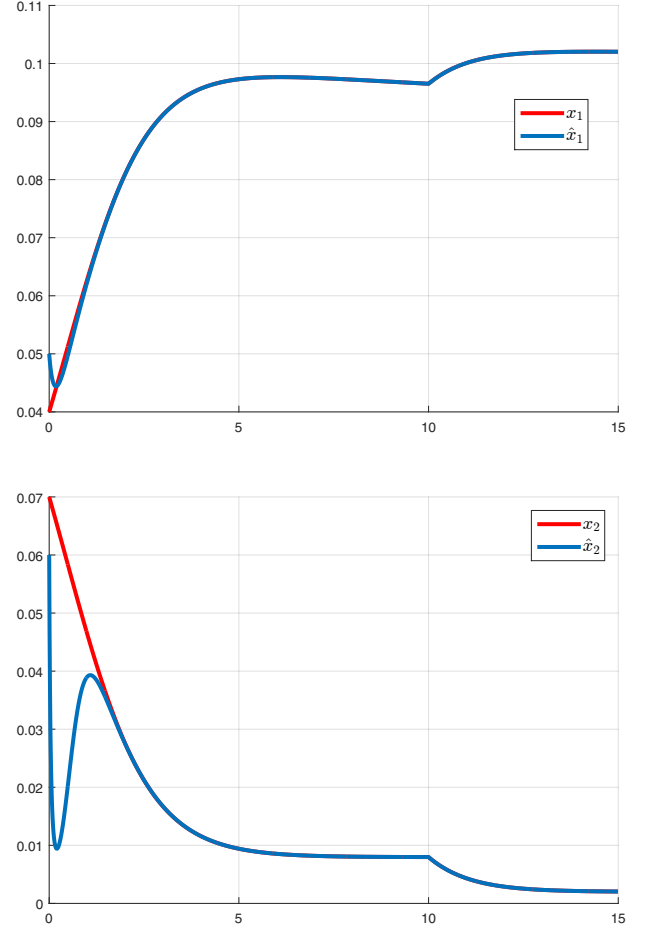
Fig. 2. Nonlinear Luenberger observer (23) for system (22) with k = 3 , \lambda_1 = 1 , \lambda_2 = 2 .
