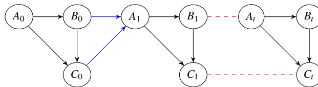
Fig. 6 Example of a dynamic Bayesian network
