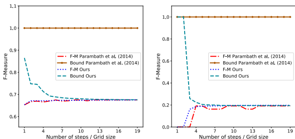
Figure 6: Training performance of CONE versus the grid approach from Parambath et al. (2014), together with their respective bounds (on Adult (left) and Abalone12 (right)). We suppose \epsilon_1 = 0 , which explains that we observe empirical values that are higher than our upper bound (on Abalone12).
