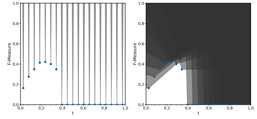
(h) Wine
