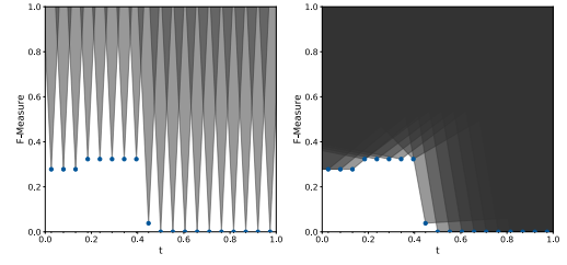
(b) Abalone10
