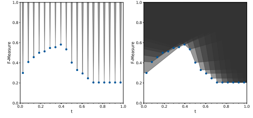
(f) Pageblocks
