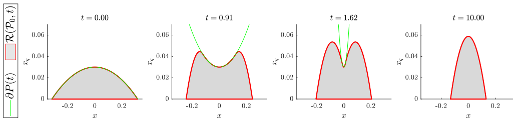
Figure 3: Time-varying paraboloid overapproximates the reachable set at different time instants t in \{0.00, 0.91, 1.62, 10.00\} for an initial maximum energetic level of x_{q,0} = 0.03 . The solution of (8) has a finite escape time and diverge at t = 1.68 . The shaded regions are the reachable set \mathcal{R}(\mathcal{P}_0, t) , the thin green lines are the boundary of the overapproximation P(t) of Theorem 1.
