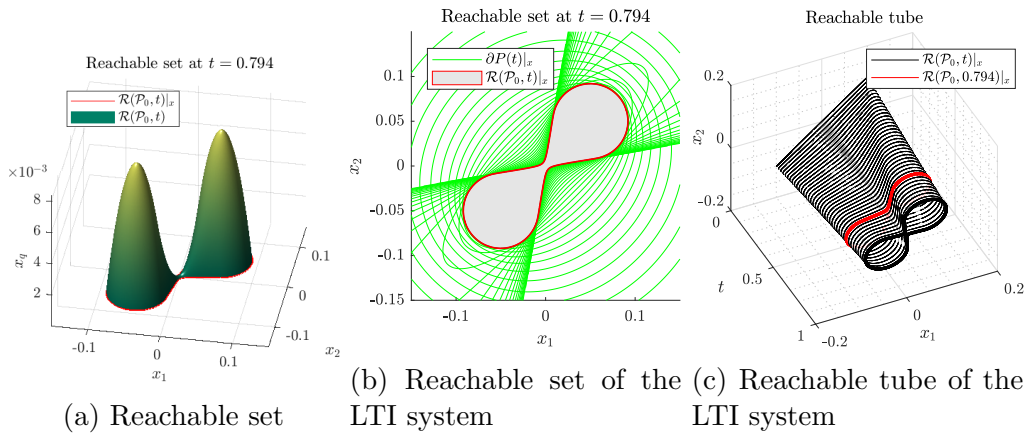
Figure 6: The green surface in (a) is the reachable set \mathcal{R}(\mathcal{P}_0, t) at t = 0.794 of \mathcal{S}(\mathcal{P}_0, t) computed using Theorem 2. Its projection over the LTI state space (x_1, x_2) (in solid red line) is shown in (b), each green line corresponds to one constraint P \in \Pi computed with Theorem 1. (c) is the reachable tube t \rightarrow \mathcal{R}(\mathcal{P}_0, t) of \mathcal{S}(\mathcal{P}_0, t) projected over the LTI state space (x_1, x_2) for t \in [0, 1] . The red section corresponds to the time t = 0.794 .
