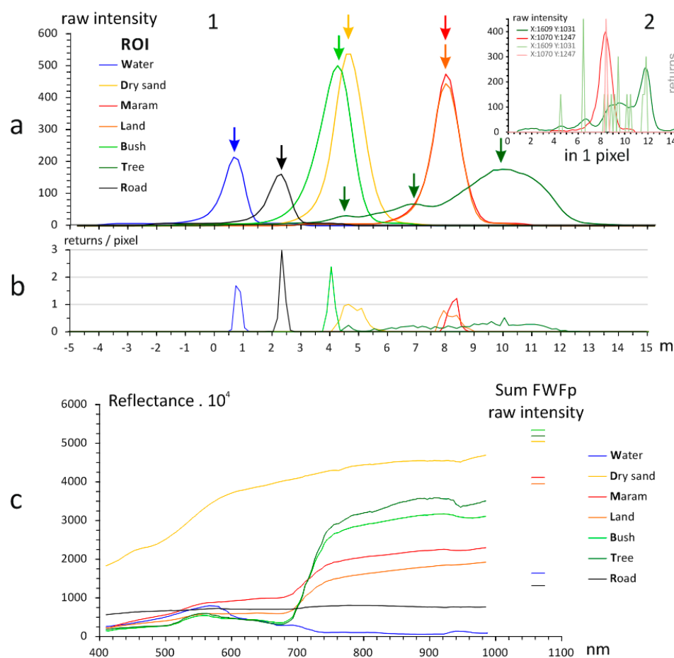
Figure 5. Comparison between echoes, FWFP and hyperspectral spectra. (a) 1: FWFP of seven regions of interest (ROI) located in Figure 1d,e; 2: FWFP and echoes of 2 pixels of sand and tree; (b) distribution of echoes in each ROI; and (c) hyperspectral reflectance of the same ROI and sum of FWFP intensity at 1064 nm.
