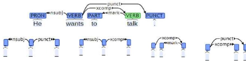
Figure 1: A dependency syntax analysis and the subsequent unlexicalized syntactic n-grams. nsbj : nominal subject, punct : punctuation, xcomp : clausal complement.
