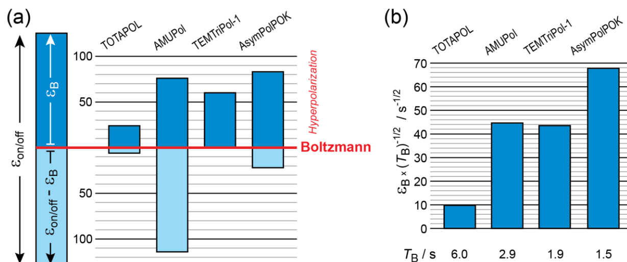
Figure 5. (a) Schematic representation of the Boltzmann hyperpolarization contribution (dark blue) to experimental \epsilon_{\text{on/off}} at 9.4 T, 10 kHz MAS frequency, and 110 K for different water soluble biradicals: TOTAPOL, AMUPol, TEMTriPol-1 and AsymPolPOK. Note that the size of the light blue bars only represents the discrepancy between \epsilon_{\text{on/off}} and \epsilon_B . It is not proportional to the amount of depolarization, which cannot be larger than the nuclear Boltzmann polarization, P_n^{\text{eq}} - P_n^{\text{off, MAS}} = (1 - \epsilon_{\text{depo}})P_n^{\text{eq}} . Experimental values for \epsilon_{\text{on/off}} and \epsilon_B (the enhancement ratio with respect to Boltzmann equilibrium) are taken from Ref. [29] for TOTAPOL and AMUPol, Ref. [34] for TEMTriPol-1 and Ref. [35] for AsymPolPOK. The biradical concentration was 12 mM for TOTAPOL and AMUPol, and 10 mM for TEMTriPol-1 and AsymPolPOK, in a standard DNP glassy matrix. Other experimental details can be found in the corresponding references. (b) Schematic representation of the sensitivity, expressed as the enhancement factor \epsilon_B divided by the square root of the hyperpolarization build-up time constant T_B , for the same biradicals as in (a). Experimental values for T_B are given below each bar and are taken from the same references as data for (a).
