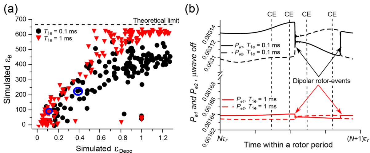
Figure 4. (a) Correlation of the simulated ^1\text{H} hyperpolarization obtained in presence of \mu\text{wave} irradiation and normalized by Boltzmann thermal equilibrium (simulated \epsilon_{\text{B}} ), with the simulated ^1\text{H} depolarization observed in absence of irradiation (simulated \epsilon_{\text{Depo}} ) for 144 different crystallite orientations of a bis-nitroxide, considering two different electron spin relaxation time constants T_{1e} of 0.1 ms (in black) and 1 ms (in red) and a MAS frequency set at 12.5 kHz. (b) Simulation of the electron polarization P_{e1} and P_{e2} (full and dashed lines) over one rotor period \tau_r after N\tau_r = 8.33 s of evolution without \mu\text{wave} irradiation (quasi-equilibrium reached) for the crystal orientation circled in blue in (a), using the same color code as in (a). Adapted from Ref. [29] with permission from the PCCP Owner Societies.
