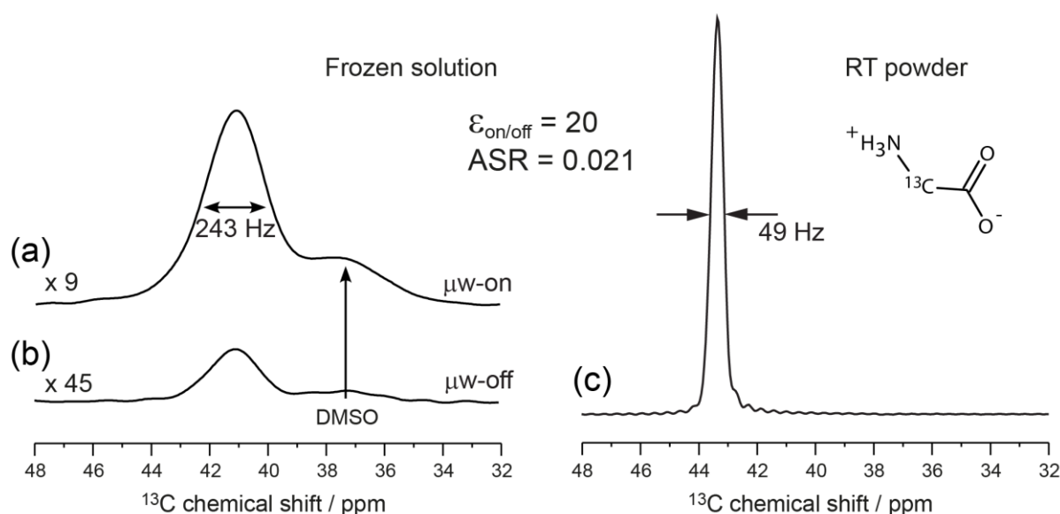
Figure 1. ^{13}\text{C} CPMAS spectra of [2-^{13}\text{C}] -glycine recorded at 9.4 T using a MAS frequency of 8 kHz. (a)-(b) Frozen solution of 0.1 M [2-^{13}\text{C}] -glycine in d_6 -DMSO/ \text{D}_2\text{O}/\text{H}_2\text{O} (6:3:1 v/v/v) with 20 mM TOTAPOL, recorded at 105 K with (a) and without (b) \mu wave irradiation for CE DNP. (c) Powder sample of [2-^{13}\text{C}] -glycine recorded at RT using conventional solid-state NMR. ASR (Absolute Sensitivity Ratio) is the ratio of (S/N)_{\sqrt{t}} between the spectra obtained under DNP and standard ssNMR conditions. Adapted with permission from Ref. [26] Copyright 2012 Wiley-VCH Verlag GmbH & Co. KGaA, Weinheim.
