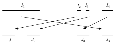
Figure 2 – An example of diffeomorphism of K_2
