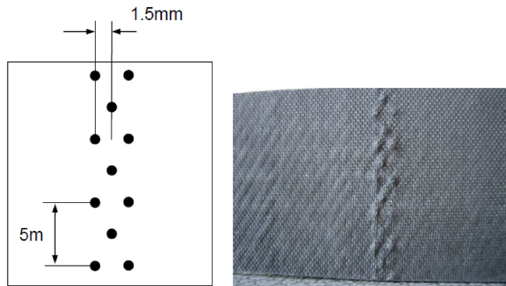
Figure N°3: Pin pattern diagram (left) and on specimen lower skin surface (right).
