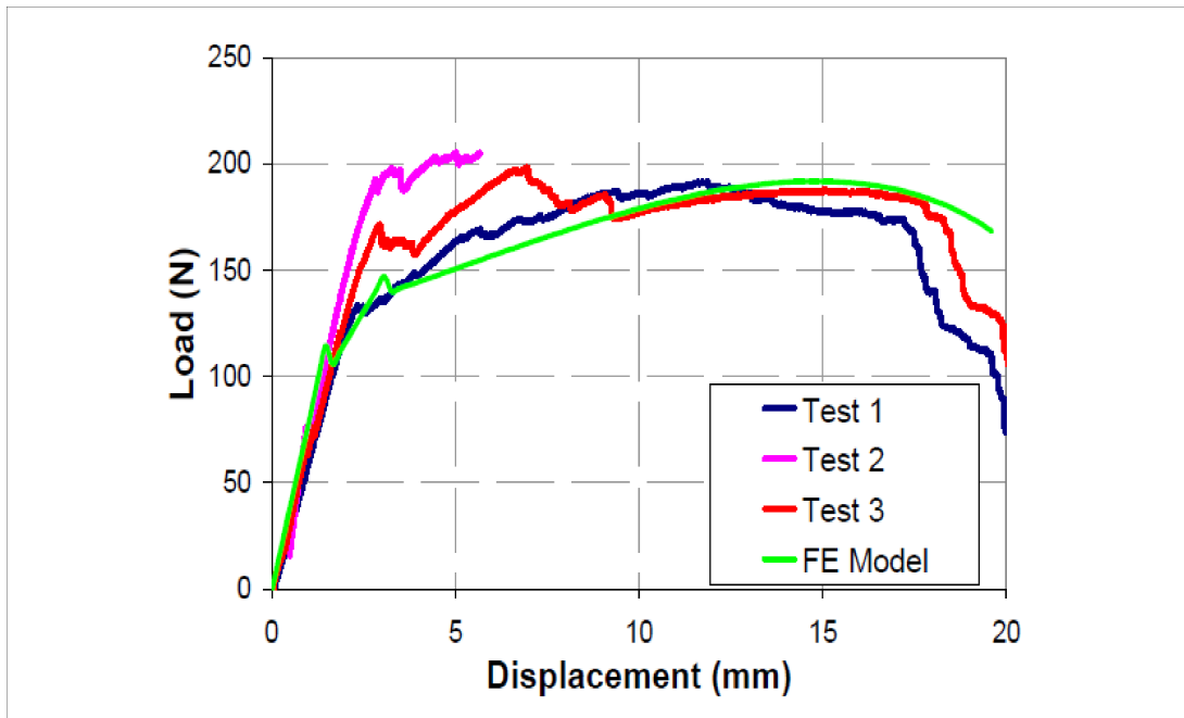
Figure N°25: Test/computation comparison for pinned T-joint under bending.
