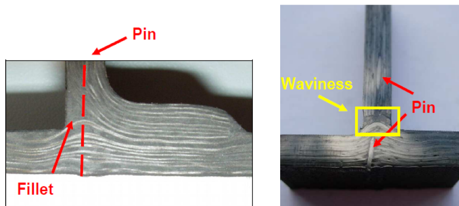
Figure N°4: Waviness created by the pin insertion.
