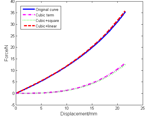
Fig. 5 Polynomial components
