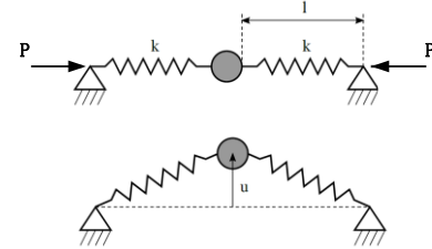
Fig.6 Negative stiffness mechanism
