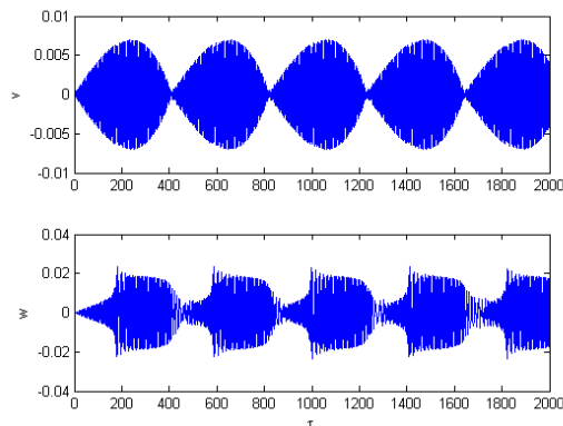
Fig.10 Strongly modulated response with G=0.1\text{mm}
