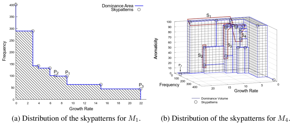
Figure 9: Analysing the skypatterns.
