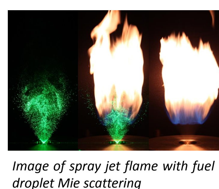
Image of spray jet flame with fuel droplet Mie scattering
