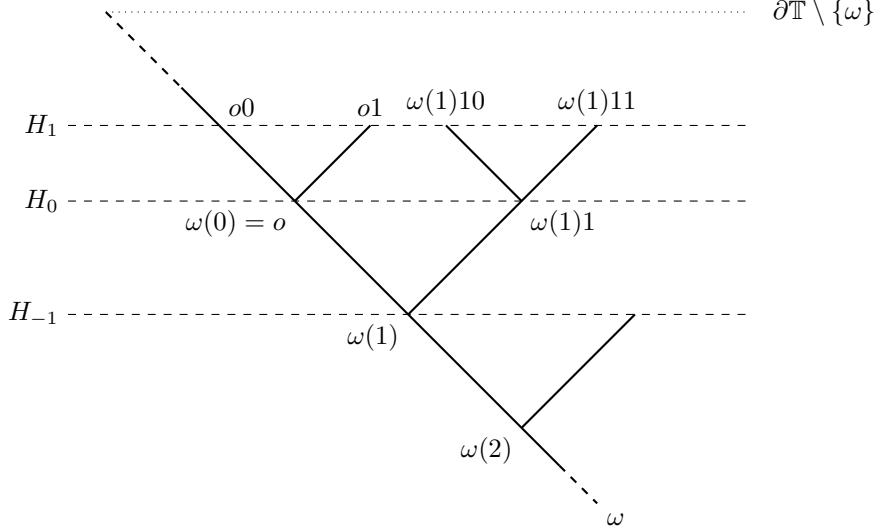
Figure 1: The affine 3-regular tree with its labelling.
