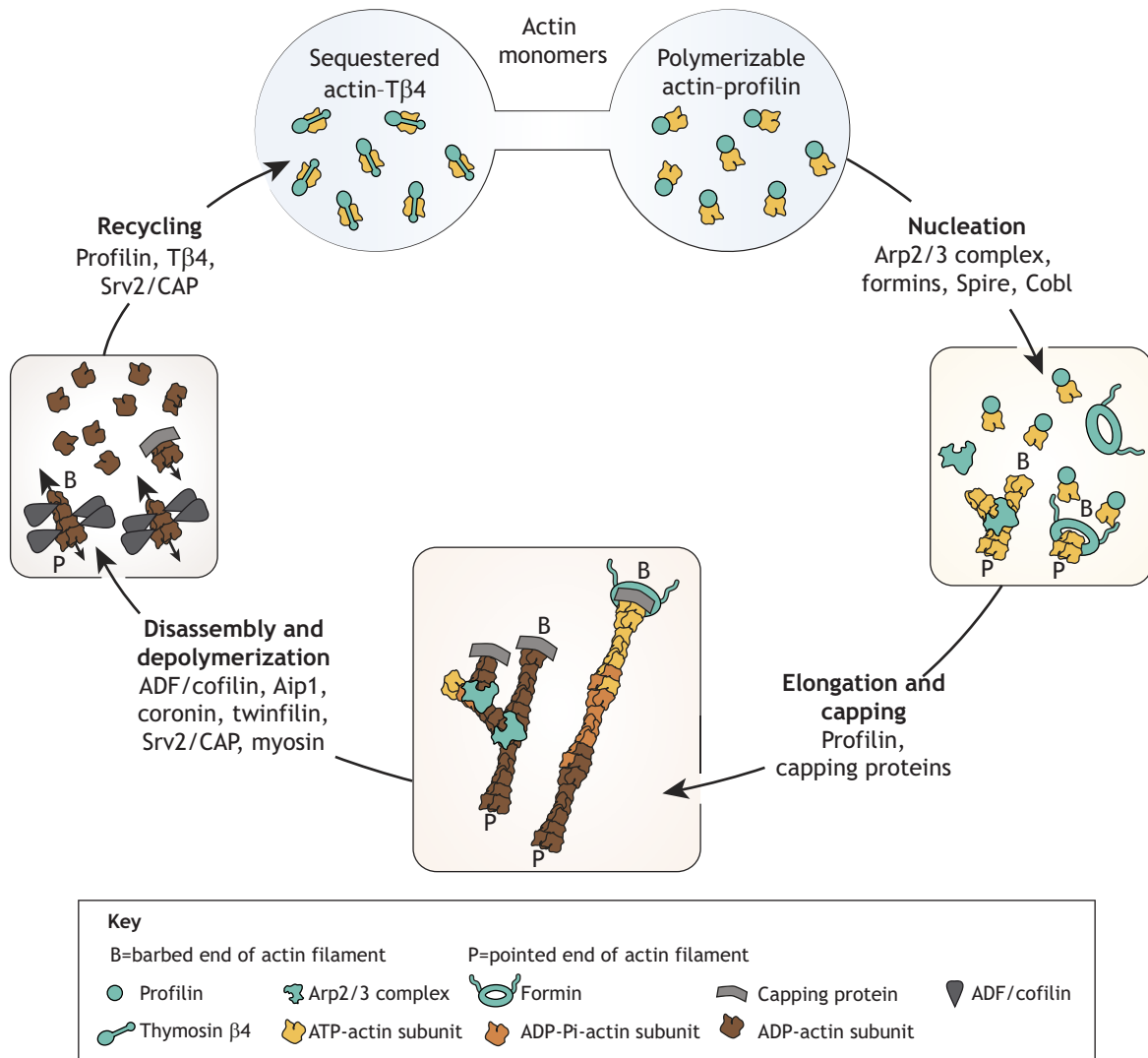
Fig. 1. The dynamic steady state of actin. Minimal steps needed to reach a dynamic steady state of different actin architectures are illustrated. Sequestered and polymerizable actin represent the pool of actin monomers. Nucleation is the formation of actin dimers or trimers. Elongation and capping modulate controlled growth of the different forms of actin organization (branched networks that are generated by the Arp2/3 complex or bundles generated by formins). Disassembly and depolymerization results in the breakdown of actin structures to monomer subunits. Recycling renews the pool of actin monomers that are charged with ATP. The different nucleotide states of actin, barbed and pointed ends and different proteins or complexes are represented by the indicated symbols.
