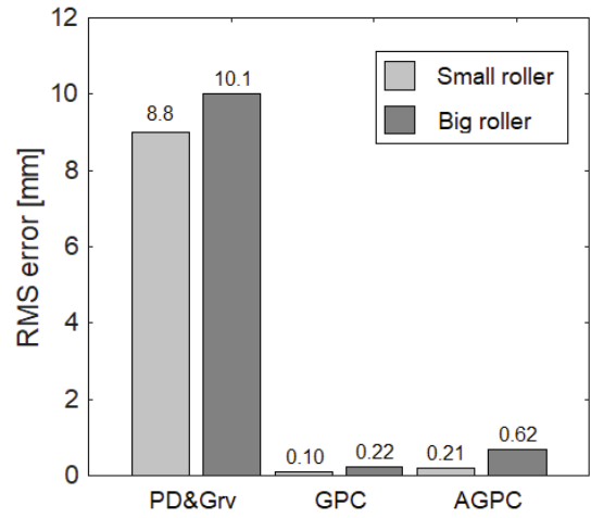
Fig. 13. RMS position error with GPC, AGPC, and PD controllers.
