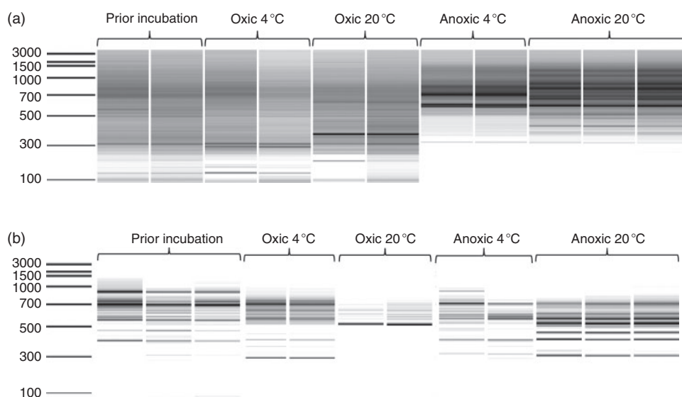
Fig. 5. ARISA profiles from streambed sediments collected in November (a) and in March (b): prior incubation and at the end of biotic incubation under oxidic conditions at 4°C, oxidic conditions at 20°C, anoxic conditions at 4°C and anoxic conditions at 20°C. Results are shown for two or three microcosm replicates. The first lane corresponds to the molecular weight DNA ladder (size are indicated in base pairs).
