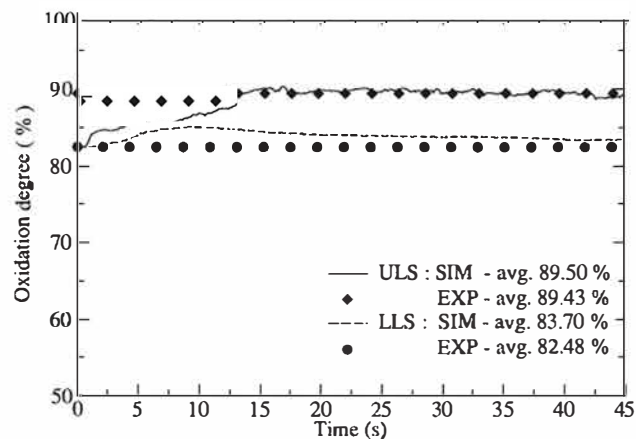
Fig. 8. Time evolution of the oxidation degree at the top of AR and in LLS.
