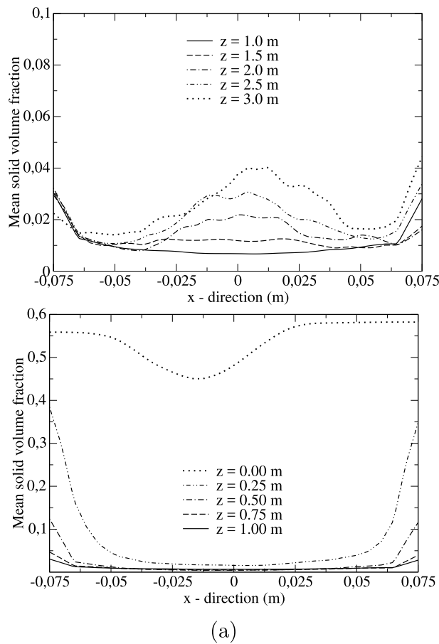
Fig. 19. Radial profiles of the time-averaged solid volume fraction (a) at different locations ( z ) within the air reactor. Local and instantaneous oxygen molar fraction (b) inside CLC (2D cut), and (c) near the wall.
