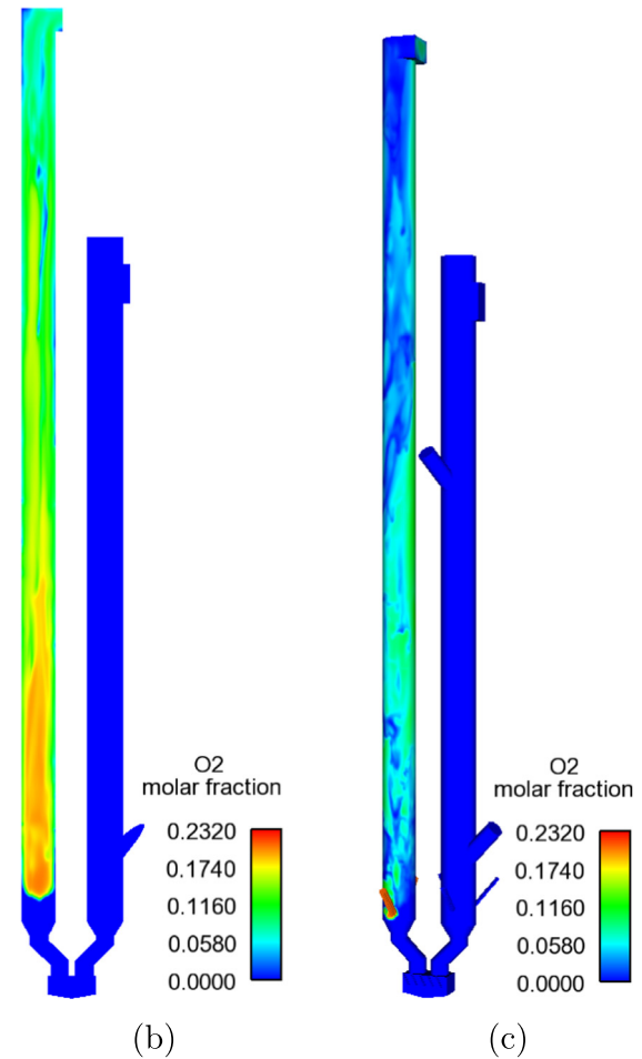
Fig. 19. Radial profiles of the time-averaged solid volume fraction (a) at different locations ( z ) within the air reactor. Local and instantaneous oxygen molar fraction (b) inside CLC (2D cut), and (c) near the wall.
