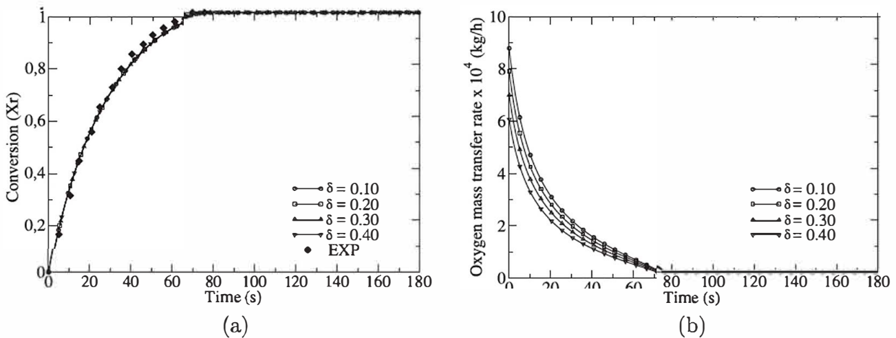
Fig. 14. 0D-model results for (a) solid conversion and (b) oxygen mass transfer rates during reduction at 1223 K and 15 %vol. of methane.
