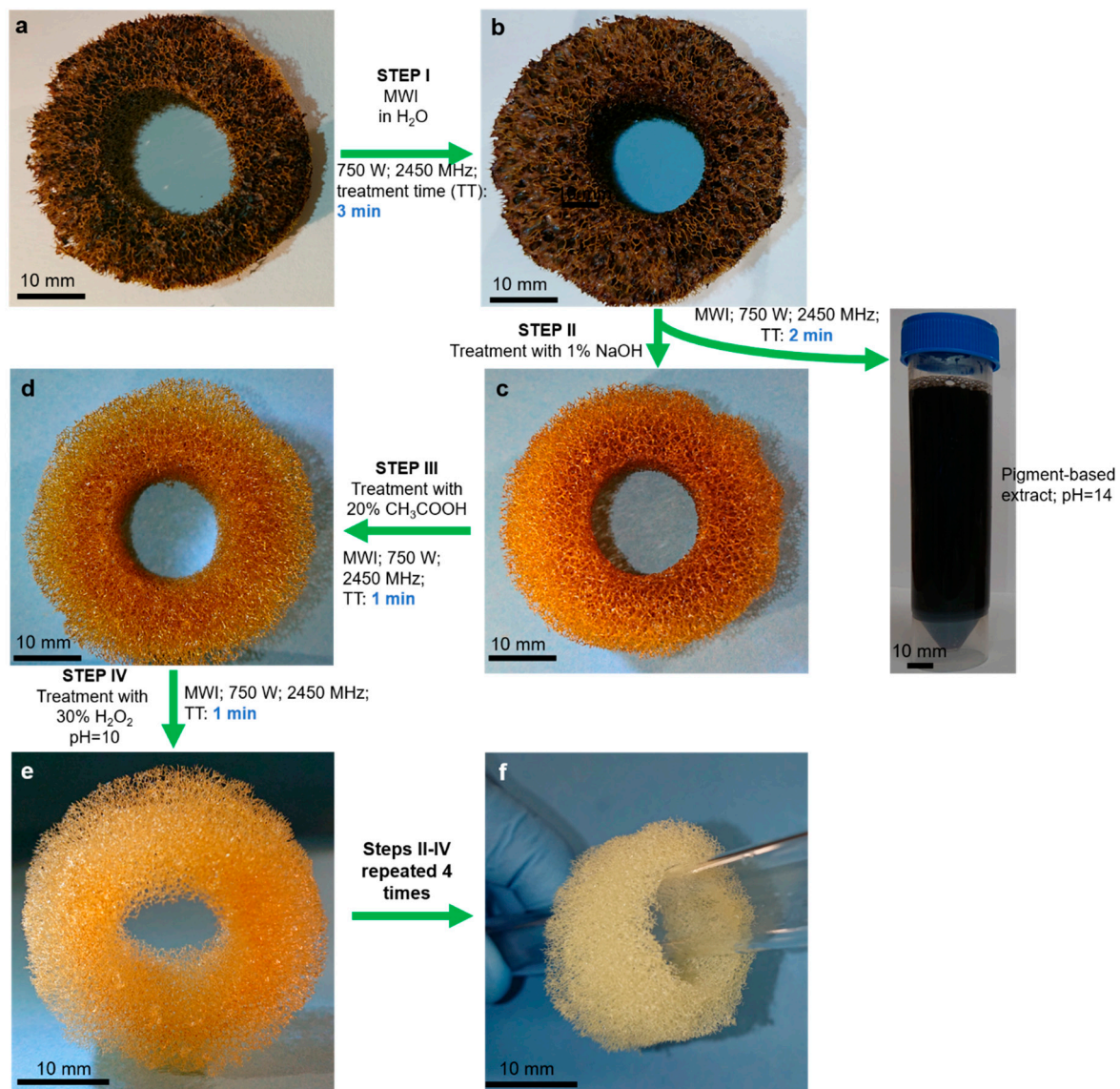
Figure 3. Schematic view of the microwave-assisted extraction of 3D chitin scaffold from a selected skeleton fragment (a) of the demosponge A. archeri . In step I, residual water soluble salts were removed by pretreatment of the sponge skeleton in distilled water under microwave irradiation (MWI) for 3 min. Afterwards, in step II (b), the sample was treated with 1% NaOH and irradiated with microwaves for 2 min. This procedure obtained both a 3D scaffold and a dark red-brownish pigment-containing extract (c). The 3D scaffold was carefully isolated and rinsed three times with distilled water to remove residual pigments. In step III, the 3D scaffolds were treated with 20% acetic acid under MWI for 1 min, and afterwards were washed in distilled water up to pH 6.8. In step IV (d,e), the sample was completely decolorized using 30% H 2 O 2 at pH~10 under MWI for 1 min and washed with distilled water up to neutral pH. Steps II–IV were repeated four times to obtain a pure, colorless, ready-to-use 3D chitinous scaffold (f).
