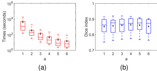
Fig. 1. Evaluation of the solver. LLCH-Exact segmentation of the 12 tumors of the clinical dataset for different grid sizes: a = \{1, 2, 3, 4, 5, 6\} . Black diamonds are the averaged values. (a) Segmentation time. (b) Dice index D(\Omega, R) of the segmented volume with respect to reference contour R .
