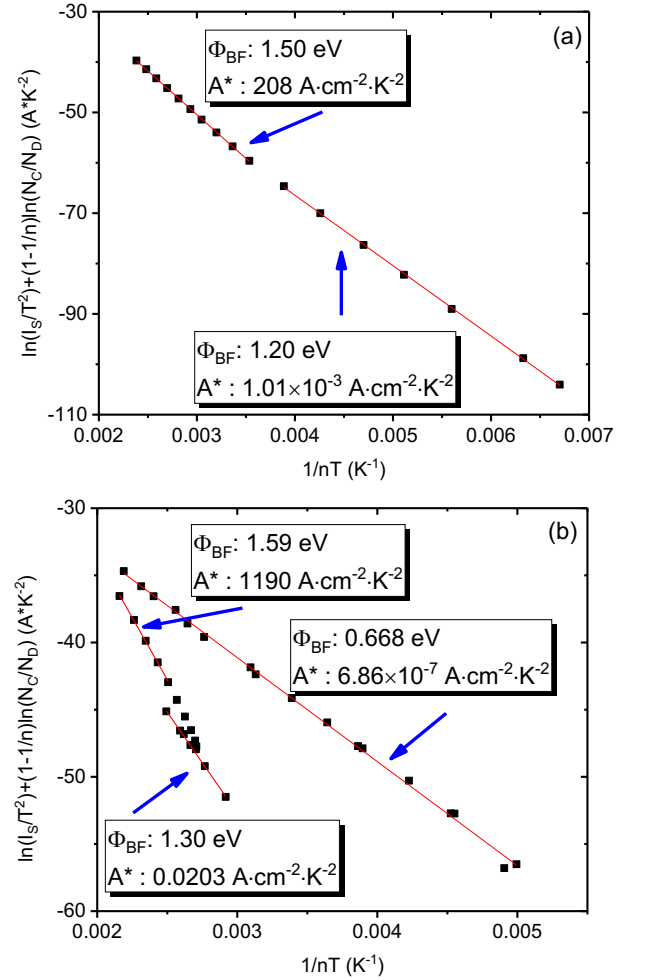
Fig. 3 Modified Richardson plot based on flat-band barrier height on diodes (a) and (b). n and I_s were calculated in the different linear zones of the I - V curves, and N_D is extracted from the C - V characteristics.
