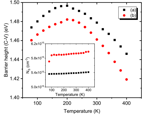
Fig. 2 SBH \Phi_B^{C-V} calculated based on the C - V characterization. The insert shows the extracted doping concentration.
