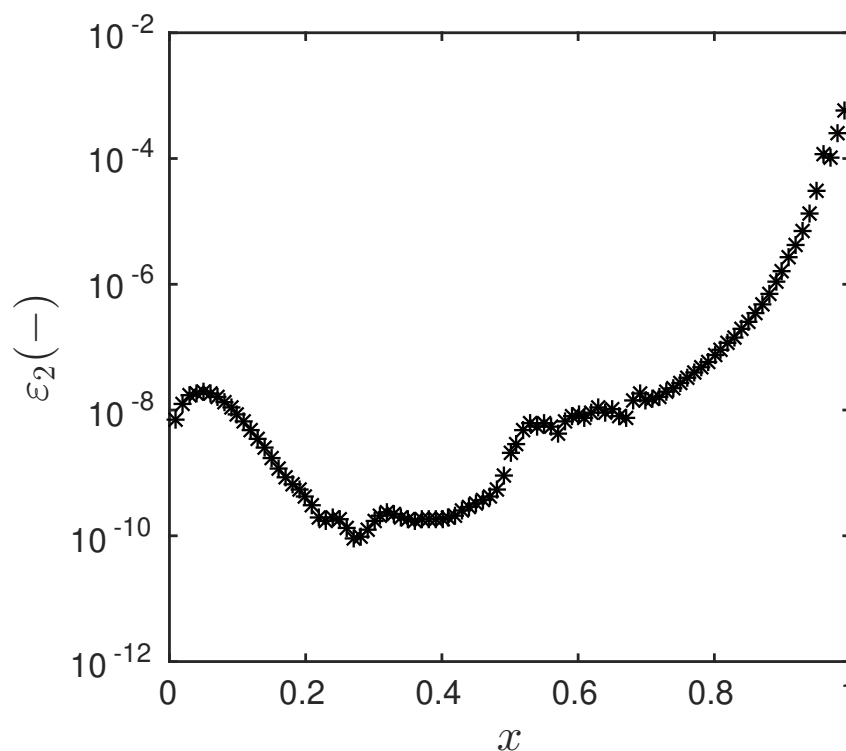
Figure 18. Error \varepsilon_2 between solutions with DIRICHLET and homogeneous NEUMANN boundary condition at x = 1 .
