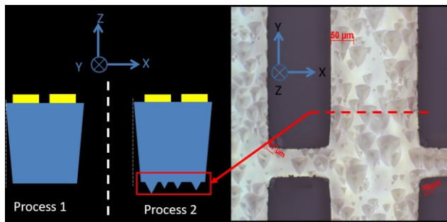
Fig. 10. Left: Schemes of the cross beam section etched with both processes. Right: photography of the back side of a resonator using wet etching and presence of pyramids with several tens of microns diameters.
