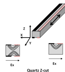
Fig. 2. Electrode scheme for the actuation of the extension mode of a Quartz Z-cut beam oriented along the Y axis. Ideally, the electrodes should be deposited on both face to optimize the electric field along X-. Real electrode system on the right.
