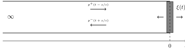
Fig. 1. Plane wave propagation in a semi-infinite duct. A loudspeaker, modeled as a flat piston, is located at z = 0 .
