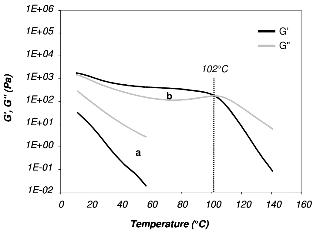
Figure 5: Conservation ( G' ) and loss ( G'' ) moduli vs temperature for blends of BPA-PO2 with neat SBM01 ( S_{22}^{9,2}B_{20}M_{58} -SB10); (a) 5 wt% SBM01; (b) 10 wt% SBM01 ( 2^{\circ}\text{C}/\text{min} , 1\text{ rad/s} ).
