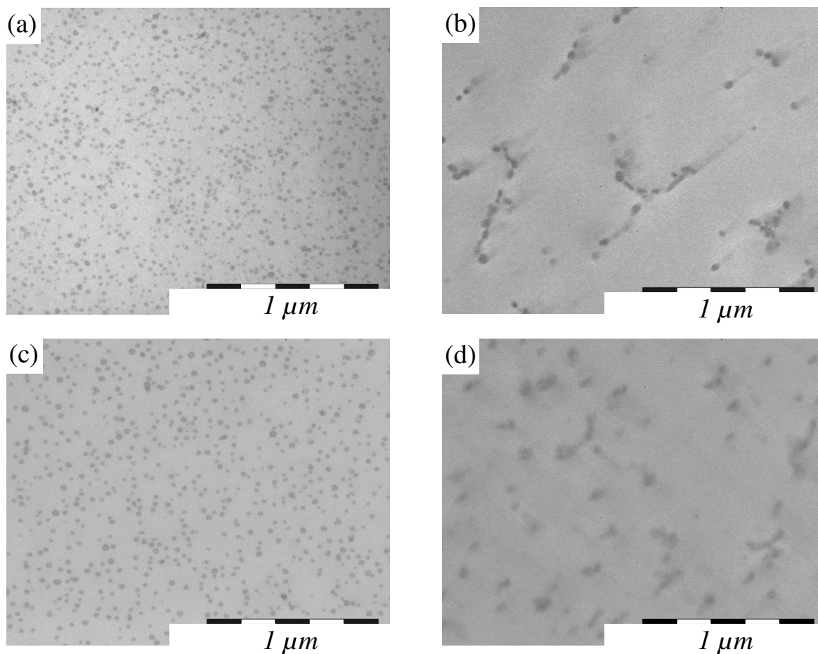
Figure 13 : TEM micrographs of the polymerized blend [IPDI/BPA-PO1 / 5 % neat SBM01] modified with various amounts of crosslinking agents: (a) IPDI/HDI = 80/20 wt%; (b) IPDI/HDI = 50/50 wt%; (c) BPA-PO1/PCL'OH = 80/20 wt%; (d) BPA-PO1/PCL'OH = 50/50 wt%
