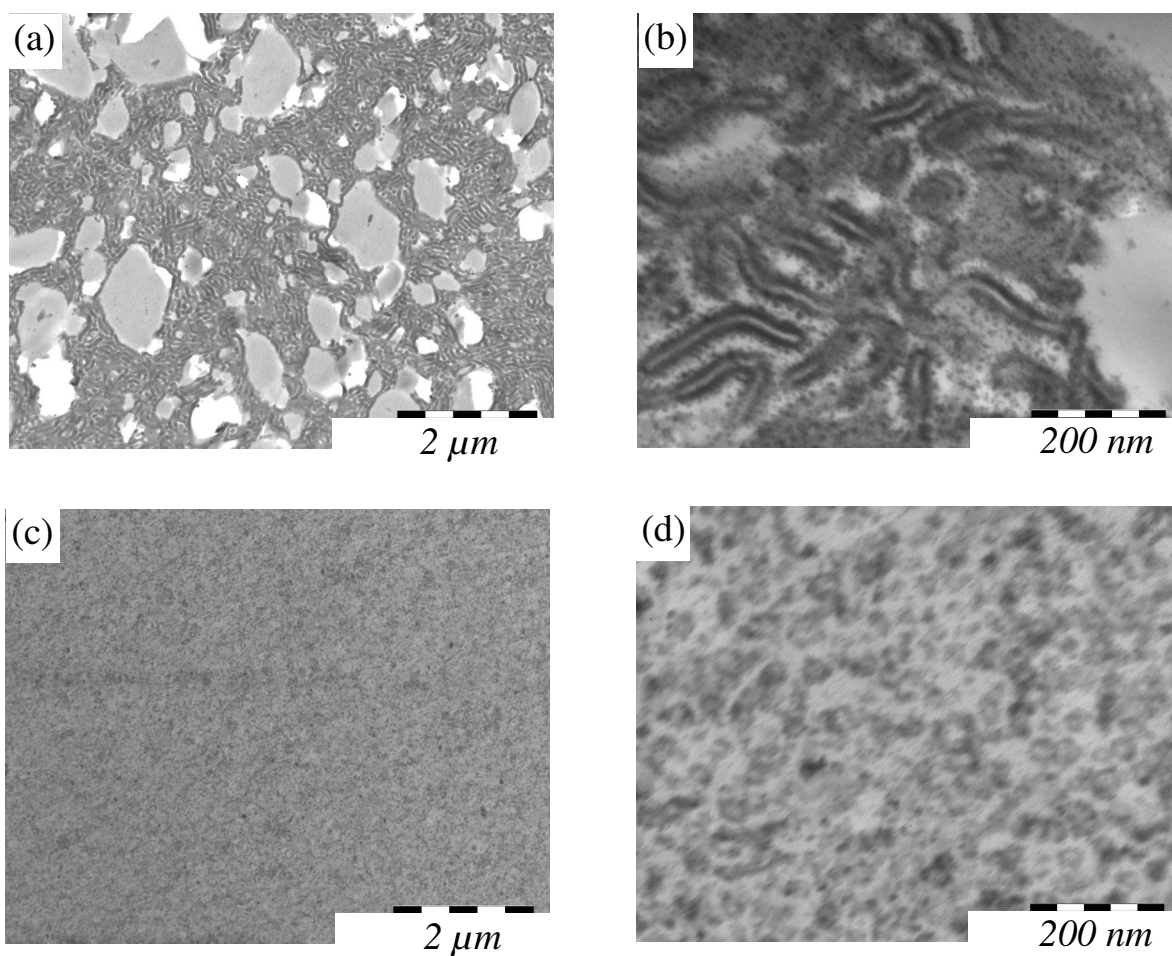
Figure 17: TEM micrographs of the SBM-modified polyurethane-urea (BPA-PO3.5/IPDI/MCDEA [OH/NCO/NH 2 1/2/1] / SBM02, 50/50 wt%); (a), (b): first process (one-stage reaction); (c), (d): second process (prepolymer process)
