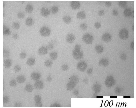
Figure 9: TEM micrographs of the polymerized blend [IPDI/(BPA-PO1/BPA-PO3.5 60/40 wt%)] / 10 wt% neat SBM01, stained with osmium tetroxide
