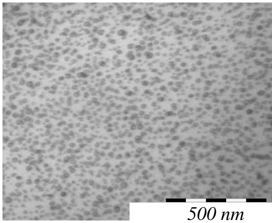
Figure 9: TEM micrographs of the polymerized blend [IPDI/(BPA-PO1/BPA-PO3.5 60/40 wt%)] / 10 wt% neat SBM01, stained with osmium tetroxide
