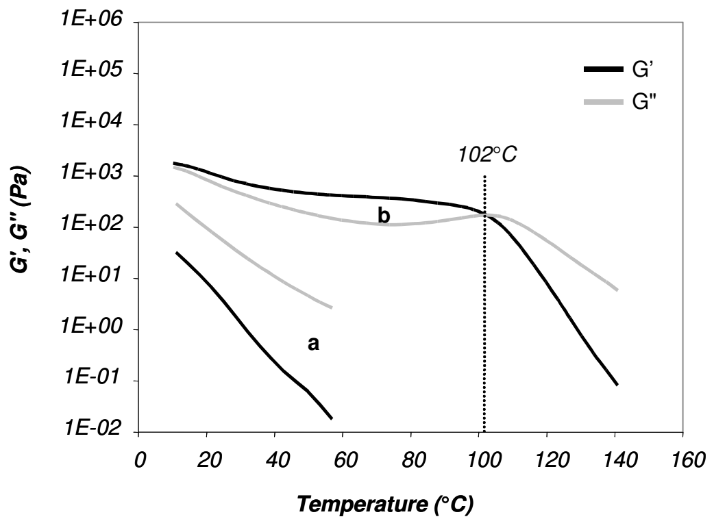
Figure 5: Conservation ( G' ) and loss ( G'' ) moduli vs temperature for blends of BPA-PO2 with neat SBM01 ( S_{22}^{9,2}B_{20}M_{58} -SB10); (a) 5 wt% SBM01; (b) 10 wt% SBM01 ( 2^\circ\text{C}/\text{min} , 1 \text{ rad/s} ).
