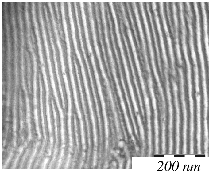
Figure 15: TEM micrograph of a neat SBM02 film obtained by solvent evaporation, stained with osmium tetroxide
