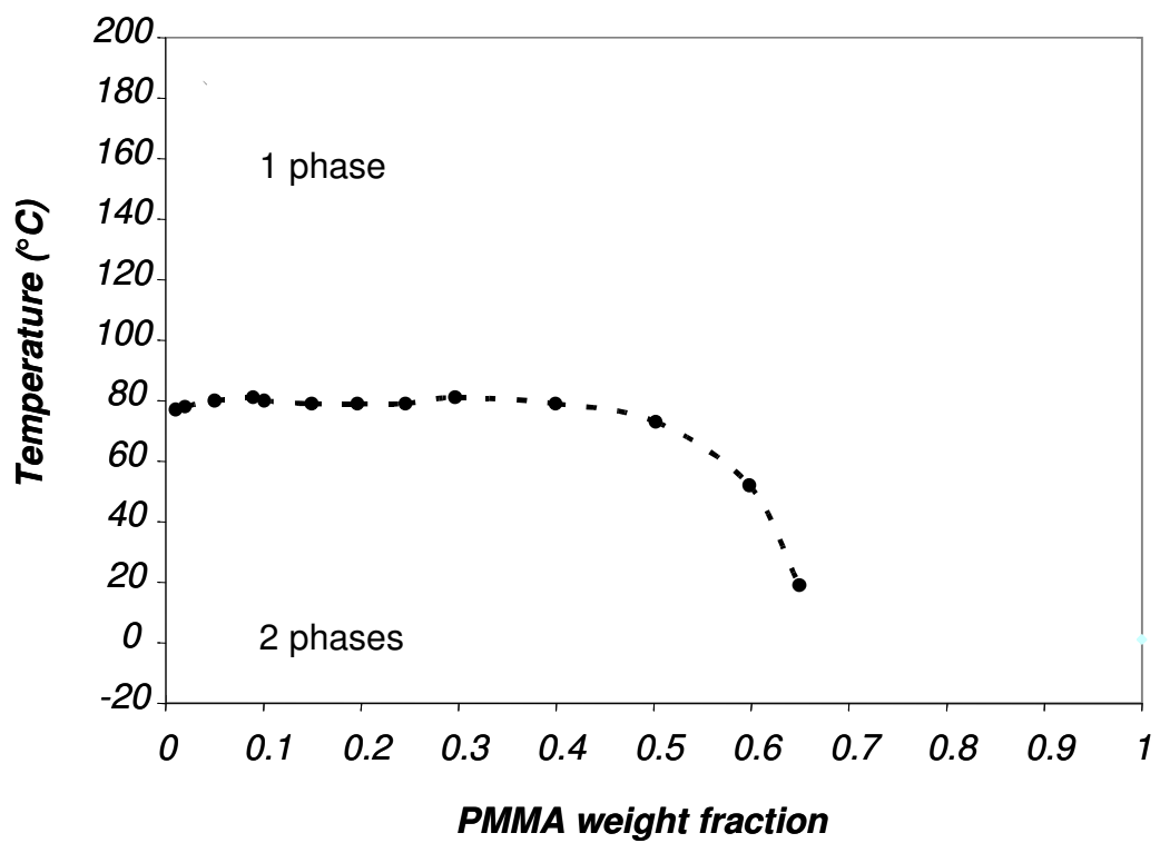
Figure 12 : Cloud point curve measured for partially miscible PCL'OH/PMMA blends
