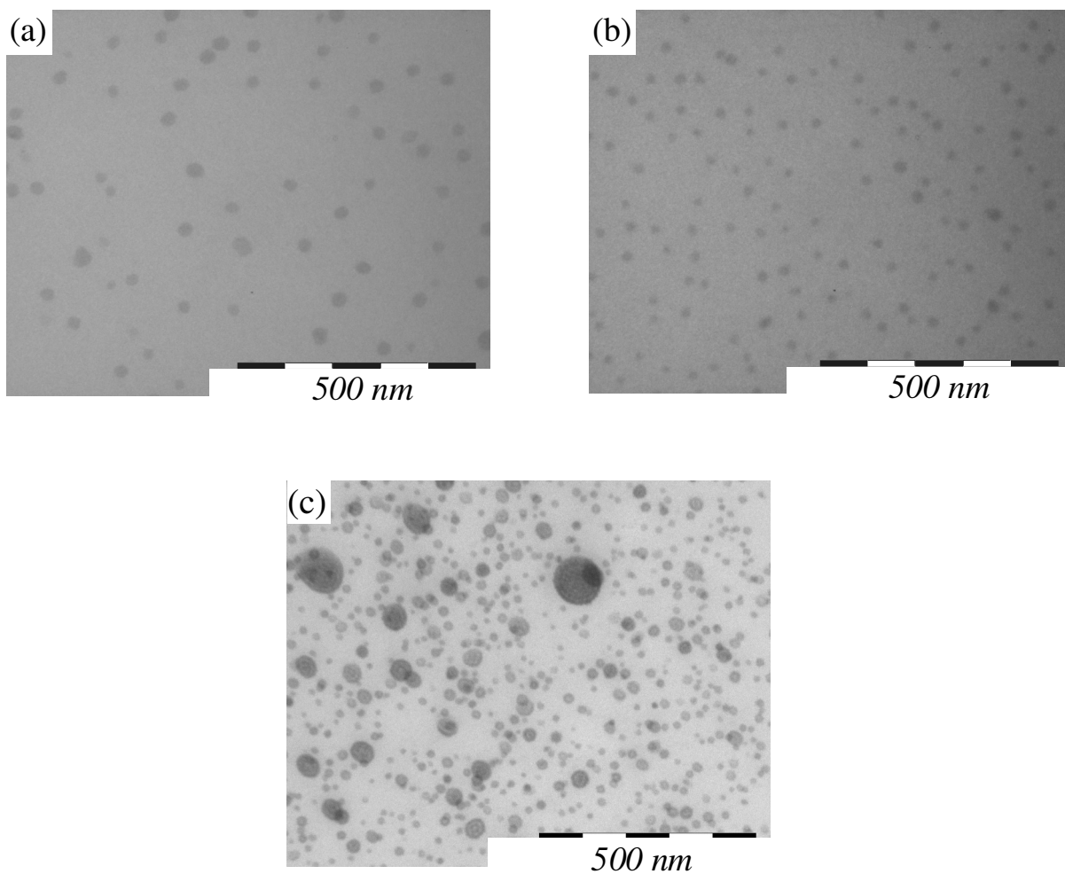
FIGURE 11 : TEM MICROGRAPHS FOR THE POLYMERIZED BLENDS ([IPDI/BPA-PO1] / 5 WT% SBM) USING (A) NEAT SBM04 ( S_{13}^{16}B_{15}M_{72} -SB17-S3); (B) PURIFIED SBM04 ( S_{13}^{16}B_{15}M_{72} ); (C) NEAT SBM03 ( S_{18}^{6,8}B_{28}M_{54} -SB52); THE SAMPLES WERE STAINED WITH OSMIUM TETROXIDE
