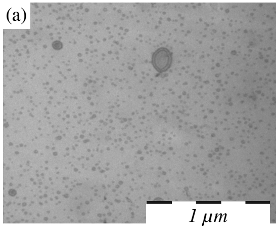
FIGURE 7 : TEM MICROGRAPHS OF THE POLYMERIZED BLENDS (A) ([IPDI/BPA-PO2] / 5 WT% NEAT SBM01) AND (B) ([IPDI/BPA-PO3,5] / 5 WT% NEAT SBM01), STAINED WITH OSMIUM TETROXIDE.
