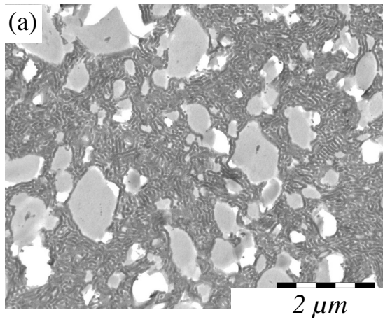
Figure 17: TEM micrographs of the SBM-modified polyurethane-urea (BPA-PO3.5/IPDI/MCDEA [OH/NCO/NH 2 1/2/1] / SBM02, 50/50 wt%); (a), (b): first process (one-stage reaction); (c), (d): second process (prepolymer process)
