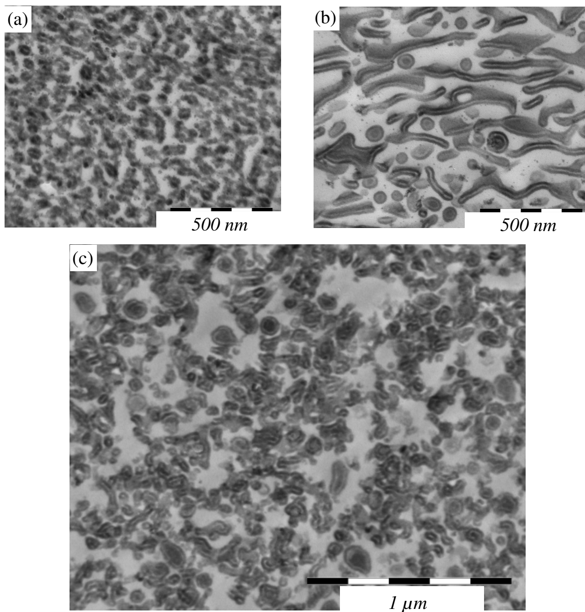
Figure 16 : TEM micrographs of the blends : (a) [IPDI/BPA-PO3.5] / 50 % neat SBM02 ( S_{23}^{9,2}B_{26}M_{51} -SB20) before reaction, (b) after reaction and (c) [IPDI/BPA-PO3.5] / 50 % purified SBM02 ( S_{23}^{9,2}B_{26}M_{51} ) after reaction
