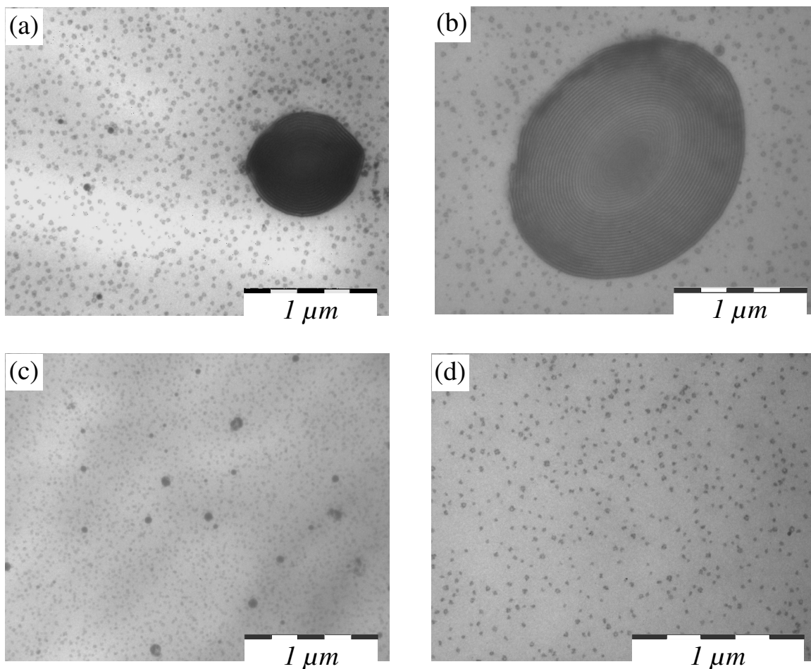
Figure 8 : TEM micrographs of the polymerized blends ([IPDI/BPA-PO3.5] / 5 wt% SBM01); (a) neat SBM, dissolution in IPDI; (b) neat SBM, dissolution in BPA-PO3.5; (c) purified SBM, dissolution in IPDI and (d) purified SBM, dissolution in BPA-PO3.5.
