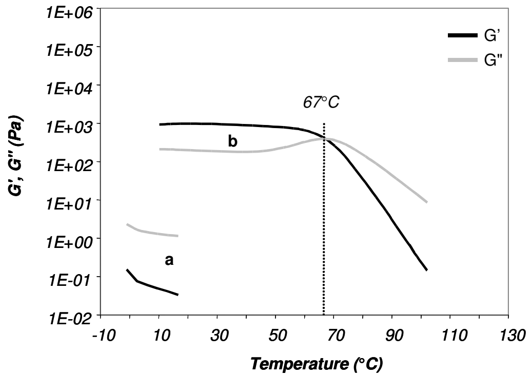
Figure 4 : Conservation ( G' ) and loss ( G'' ) moduli vs temperature for blends of XDI with neat SBM01 ( S_{22}^{9,2}B_{20}M_{58} -SB10); (a) 5 wt% SBM01; (b) 10 wt% SBM01 ( 2^{\circ}\text{C}/\text{min} , 1 \text{ rad/s} ).
