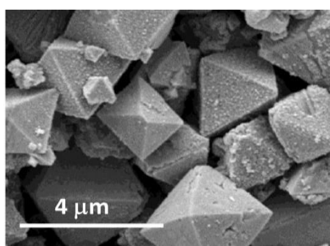
Figure 1. SEM image of SnO 2 octahedra.
