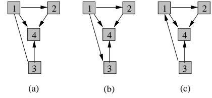
Fig. 3. (a) The partial orientation \mathbb{D}' obtained by Algorithm 1; (b) and (c) valid orientations obtained by assigning any direction to the dominated edge t_1t_3 .
