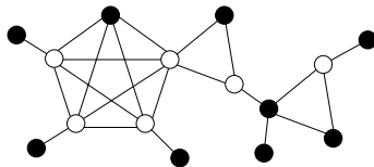
Figure 1: A block graph B (the black vertices form an identifying code of B ).
