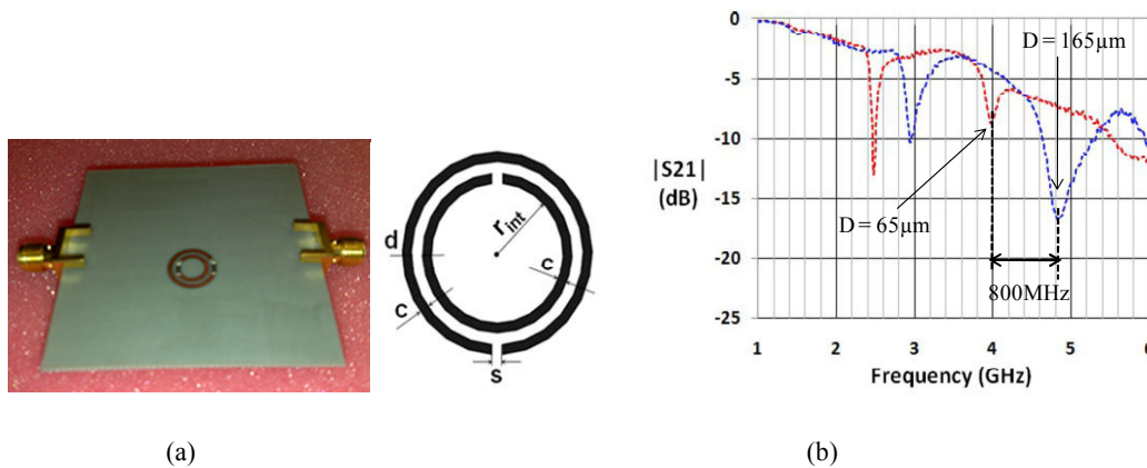
Fig. 6 : 3GHz temperature sensor prototype on 787µm thick Neltec substrate (a) Sensor view (rint=2.5mm, c=1mm, d=0.5mm, s=1mm) ; (b) S21 magnitude versus frequency for uniform cantilever displacement.
