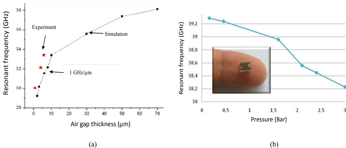
Fig. 2 : Resonant frequency versus (a) air gap (with 300µm thick silicon membrane and uniform membrane displacement) ; (b) pressure (with 45µm thick silicon membrane).
