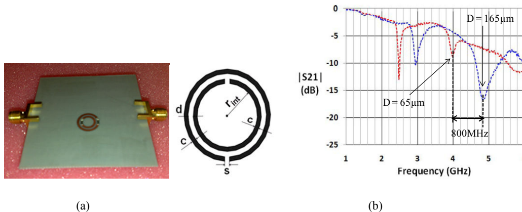
Fig. 6 : 3GHz temperature sensor prototype on 787 \mu m thick Neltec substrate (a) Sensor view ( r_{int} =2.5mm, c =1mm, d =0.5mm, s =1mm) ; (b) S21 magnitude versus frequency for uniform cantilever displacement.
