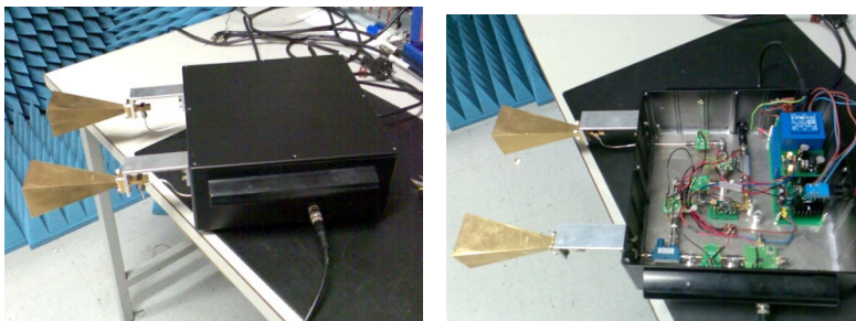
Fig. 11 : Photographies of the fabricated Radar prototype
