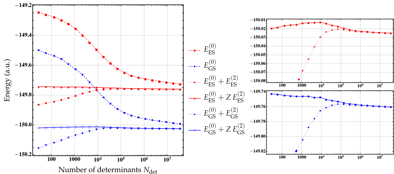
FIG. 3. Energy convergence of the ground state (GS, in blue) and excited state (ES, in red) of CN3 with respect to the number of determinants N_{\text{det}} in the reference space. The zeroth-order energy E^{(0)} (dashed), its second-order corrected value E^{(0)} + E^{(2)} (dotted) as well as its renormalized version E^{(0)} + Z E^{(2)} (solid) are represented. See Table I for raw data.
