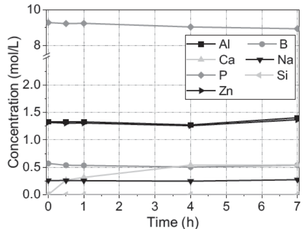
Fig. 11. Variations of the concentration of aluminum, boron, calcium, sodium, phosphorus, silicon and zinc in the liquid phase over the first 7 h of hydration.
