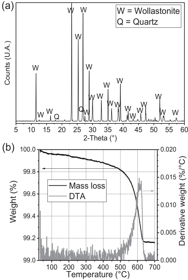
Fig. 1. Mineralogical characterization of the cement powder by X-ray diffraction (a) and thermogravimetry analysis (b).
