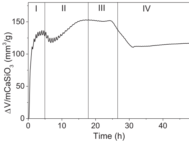
Fig. 14. Measured volume variation during hydration of wollastonite.
