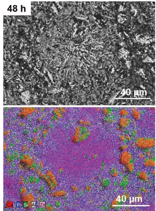
Fig. 10. SEM observation of the polished section of a 48 h-old sample. Top: BSE image; Bottom: elemental mapping (Ca, Al, P, Si, Zn).
