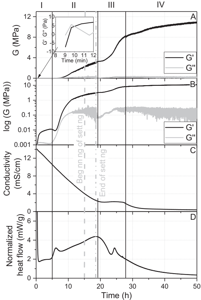
Fig. 3. Evolution of the viscoelastic parameters (A and B), electrical conductivity (C) and heat flow (D) with ongoing hydration.
