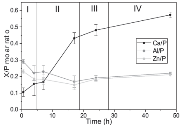
Fig. 6. Evolution of the Ca/P, Al/P and Zn/P molar ratios of the amorphous phosphate phase.
