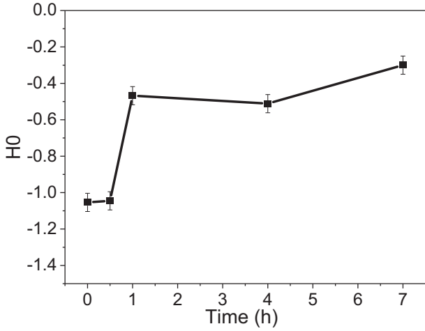
Fig. 2. Evolution of the acidity function of the interstitial solution up to 7 h of hydration.
