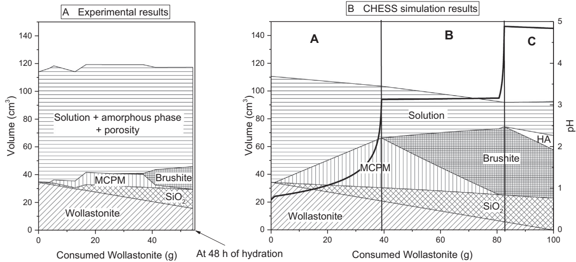
Fig. 13. Volume and phase evolution during the hydration of wollastonite by a phosphoric acid solution A- Experimental results, B- Modelling results.
