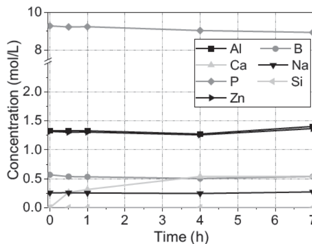
Fig. 11. Variations of the concentration of aluminum, boron, calcium, sodium, phosphorus, silicon and zinc in the liquid phase over the first 7 h of hydration.
