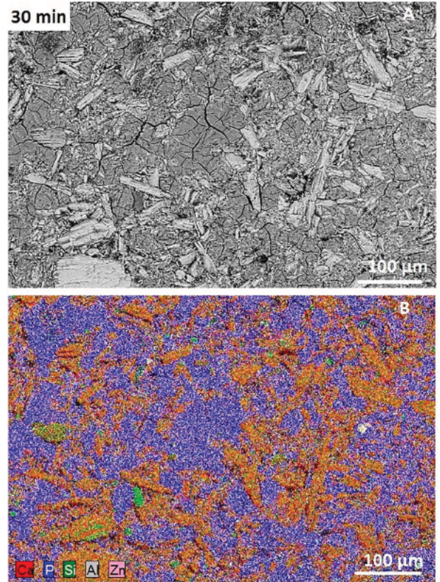
Fig. 5. SEM observation of the polished section of a 30 min-old sample. Top: BSE image; Bottom: elemental mapping (Ca, Al, P, Si, Zn).
