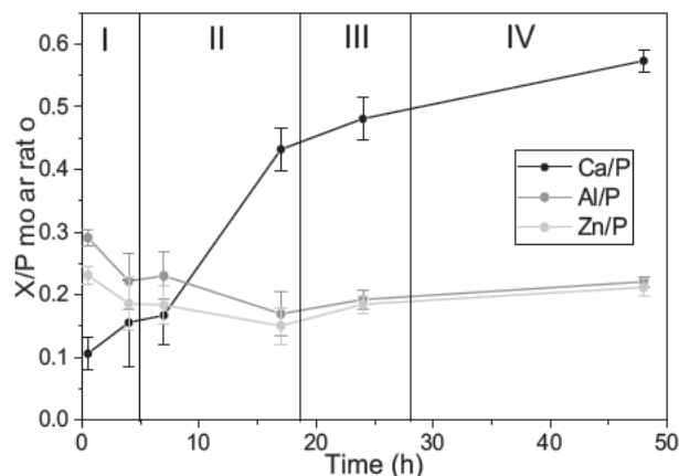
Fig. 6. Evolution of the Ca/P, Al/P and Zn/P molar ratios of the amorphous phosphate phase.
