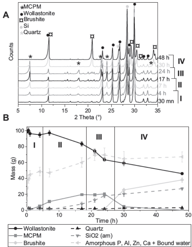
Fig. 4. Evolution of the phase assemblage with ongoing hydration: (a) X-ray diffraction patterns; (b) phase evolution assessed from Rietveld and elemental analysis as well as mass balance calculations.
