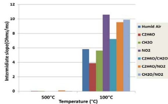
Fig.12. Representation of the intermediate slopes under different gases at the 8 th cycle in “Ohms/ms” according to the temperature of the sensors [11].
