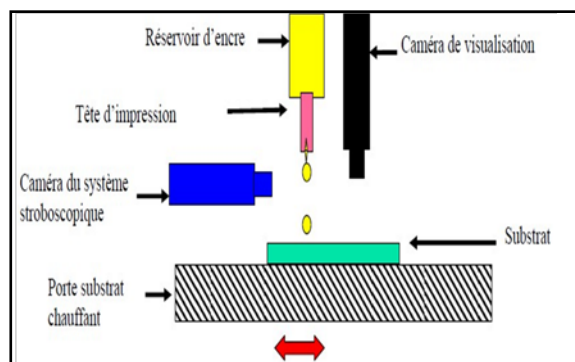
Fig.2. Schematic diagram of the inkjet machine.
