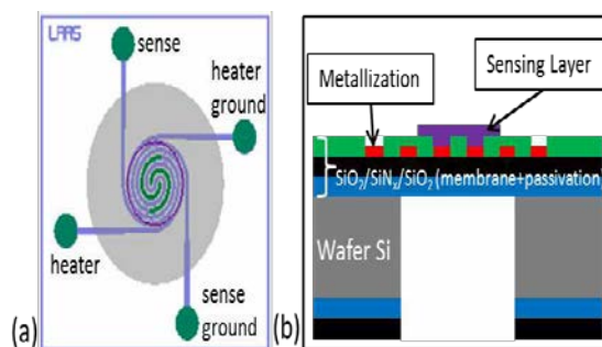
Fig.3. Micro-hotplate gas sensor: (a) Top view, (b) Cross sectional view.
