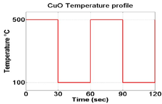
Fig.4. CuO temperature profile.
