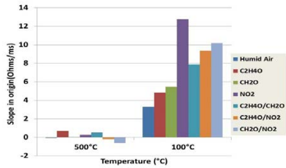
Fig.11. Representation of the slopes at the origin under different gases of the 8 th cycle in “Ohms/ms” according to the temperature of the sensors [11].
