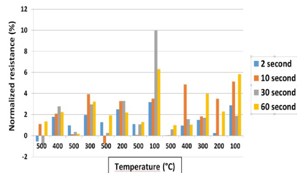
Fig.6. Representation of the normalized resistance of CuO sensor under 300ppb of NO 2 at different temperature stages.
