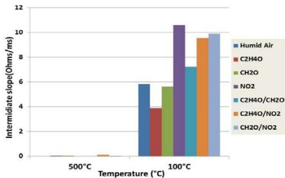
Fig.12. Representation of the intermediate slopes under different gases at the 8 th cycle in “Ohms/ms” according to the temperature of the sensors [11].
