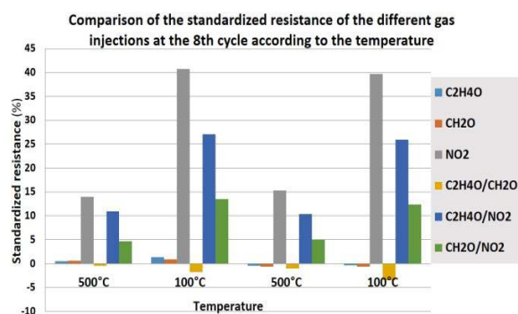
Fig.14. The normalized resistance of the different gas injections at the 8 th cycle according to the temperature [11].
