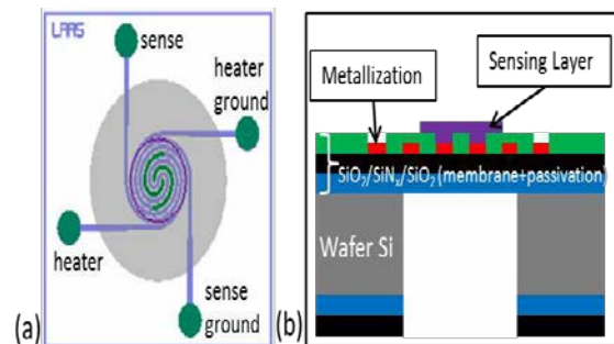
Fig.3. Micro-hotplate gas sensor: (a) Top view, (b) Cross sectional view.
