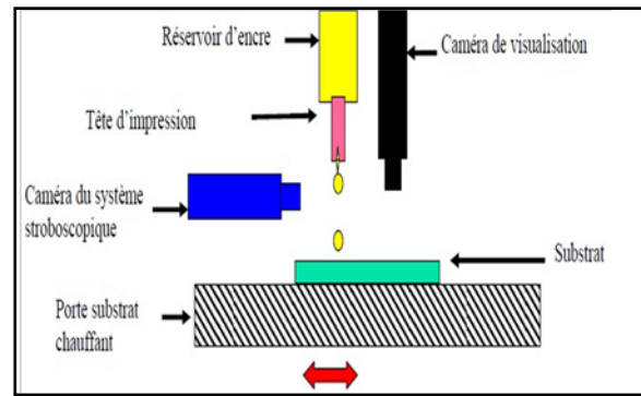
Fig.2. Schematic diagram of the inkjet machine.
