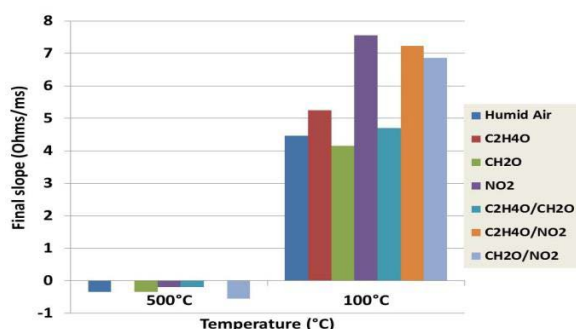
Fig.13. Representation of the final slopes under different gases at the 8 th cycle in “Ohms/ms” according to the temperature of the sensors [11].
