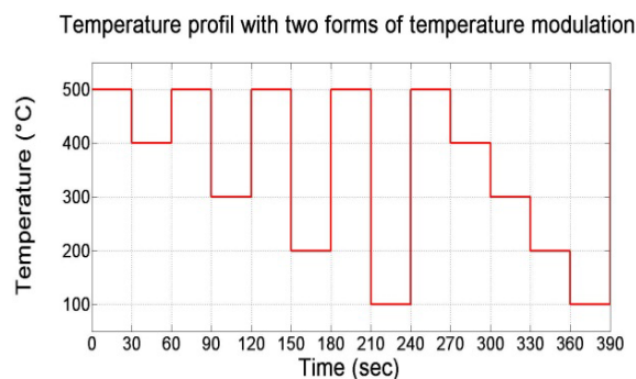
Fig.5. Form of temperature modulation.
