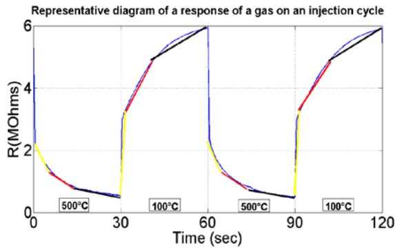
Fig.9. Representative diagram of a response of a gas sensor during an injection cycle and showing the 3 domain slopes [11].
