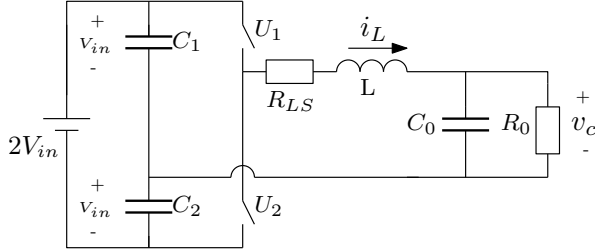
Fig. 1. Half-bridge inverter.
