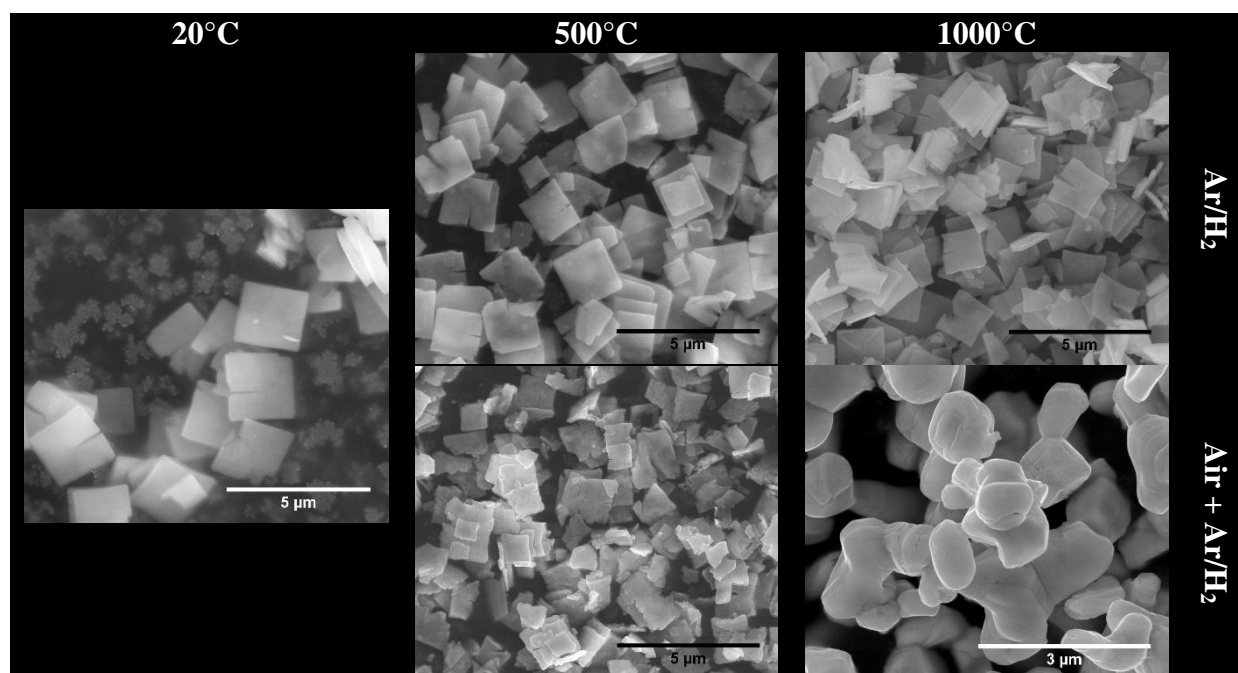
Figure 7. SEM observations of \text{U}(\text{C}_2\text{O}_4)_2 \cdot 2\text{H}_2\text{O} and of the oxide powders obtained after heating treatment at 500°C and 1000°C following the two thermal cycles considered.
