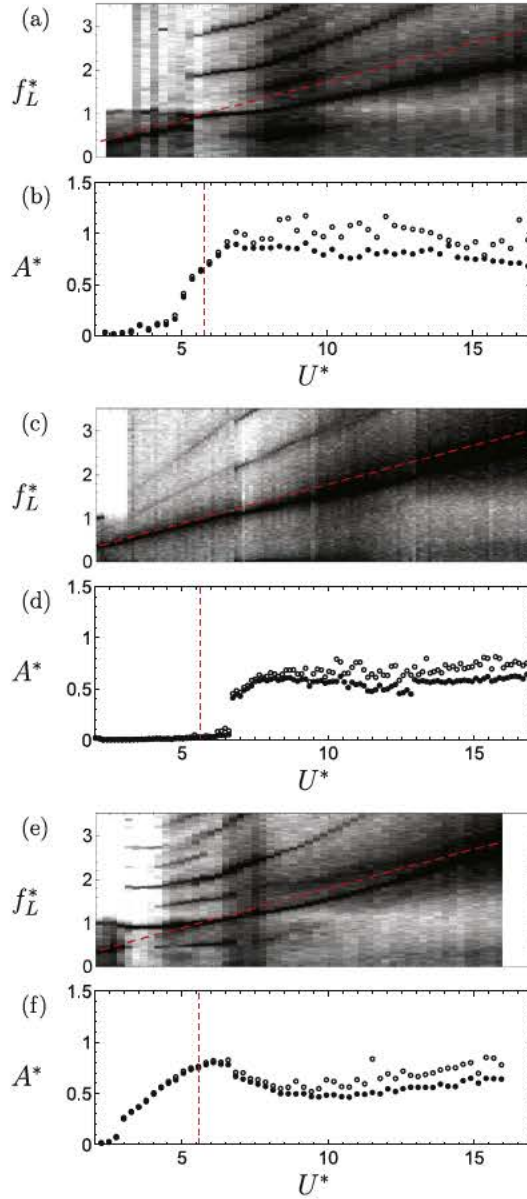
Fig. 14. (a),(c) and (e): Logarithmic-scale reduced frequency power spectrum contours of the lift coefficient f_L^* and (b),(d) and (f): the normalized amplitude response A^* for \alpha = 20^\circ , 45^\circ and 50^\circ , respectively, as a function of U^* . Open and filled markers indicate A_{\max}^* and A_{10}^* responses, respectively; the slope dashed lines denote the Strouhal vortex shedding frequency; the vertical dashed lines denote U^* = 1/Sr in the amplitude response plots.
