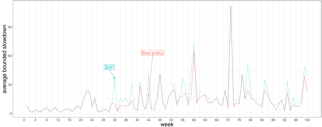
Fig. 2. Comparing SAF, the best pure policy on average, with the best pure policy for every week for the SDSC-SP2 trace.
