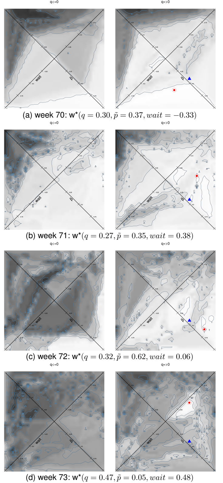
Fig. 4. Visualization of the search space for 4 consecutive weeks 70, 71, 72, and 73. The two diagonal axis represent \tilde{p} and wait . The lighter the area is, the better the performance (lower average BSLD ). The optimal area change from one week to the next. The red dot (in the lightest area) represents \mathbf{w}^* and the blue triangle represents \mathbf{w}_{train} .
