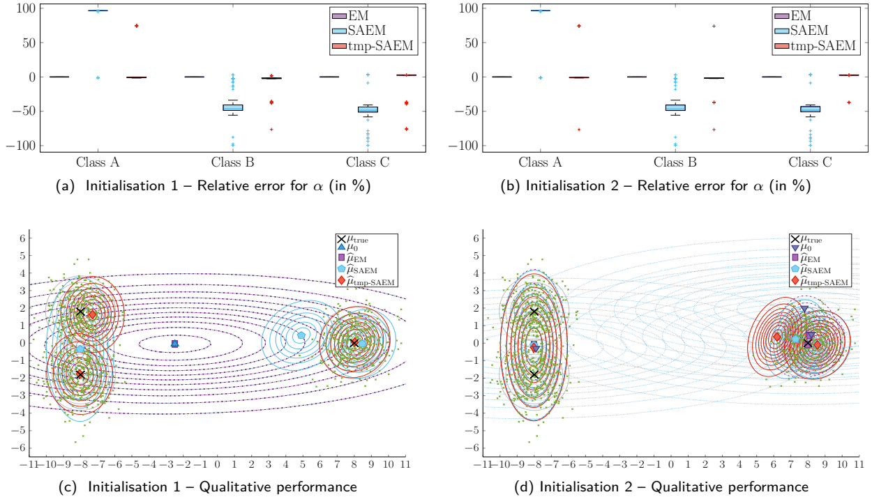
Figure 7: Performance of the estimation for the dataset III . Figs. 7a and 7b: Relative error (expressed as a percentage) for the weights \alpha , for 100 runs and n = 1000 , according to the type of initialization.
