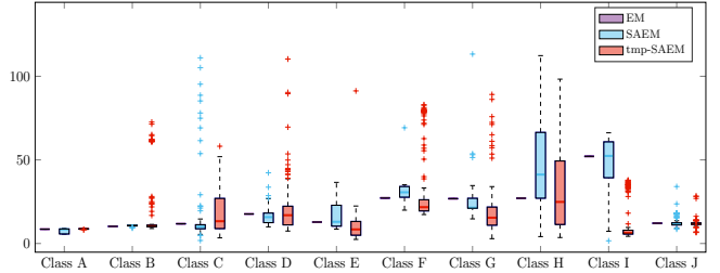
(c) KL distance between the true \Sigma and the estimated ones
