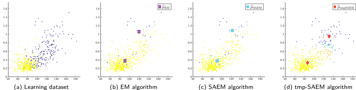
Figure 11: Weastbreast Cancer Wisconsin Dataset – Situation 2 . Fig. 11a: Learning dataset colored according to the true label. Figs. 11b, 11c and 11d: Observed data colored according to their mean probability of belonging to the Malignant class. Tempering scheme: a = 0, b = -1, c = 1, r = 1 .
