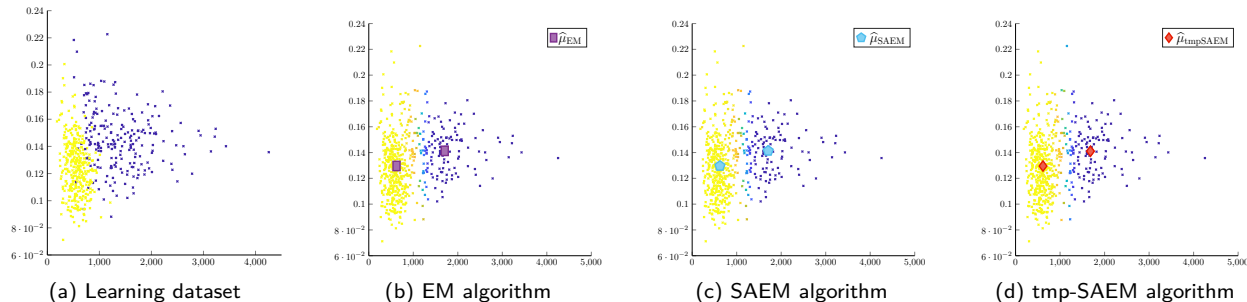
Figure 10: Weastbreast Cancer Wisconsin Dataset – Situation 1 . Fig. 10a: Learning dataset colored according to the true label: Malignant in yellow and Benign in dark blue. Figs. 10b, 10c and 10d: Observed data colored according to their mean probability of belonging to the Malignant class: from 0 in dark blue to 1 in yellow. Average probability taken over 100 runs. Tempering scheme: a = 0, b = -1, c = 1, r = 1 .
