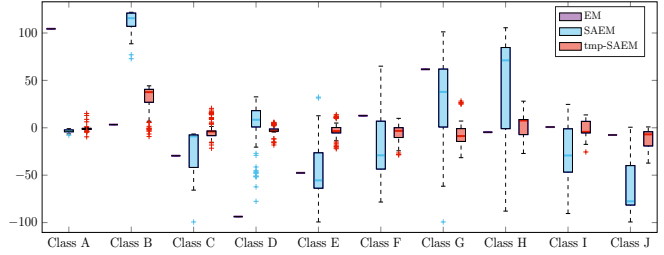
(a) Relative error (expressed as a percentage) for \alpha
