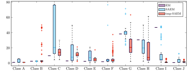
(b) Relative error (expressed as a percentage) for \mu
