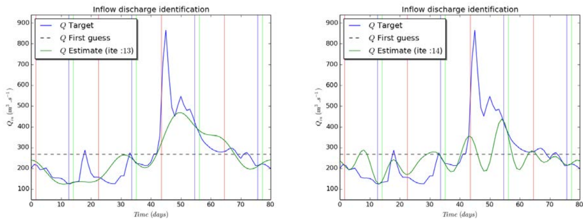
FIGURE 5.2. Garonne river, Scenario 1. Discharge identification with Fourier series with: (Left) N_{FS} = 5 , e_2^{T_{obs}}(Q_{in}^{estimate}) = 17.1\% . (Right) N_{FS} = 10 , e_2^{T_{obs}}(Q_{in}^{estimate}) = 16.2\% . Vertical lines corresponds to the time observations (blue for Group 1, red for Group 2 and green for Group 3). The horizontal dotted line corresponds to the first guess Q_{in} = 268 \text{ m}^3/\text{s} .
