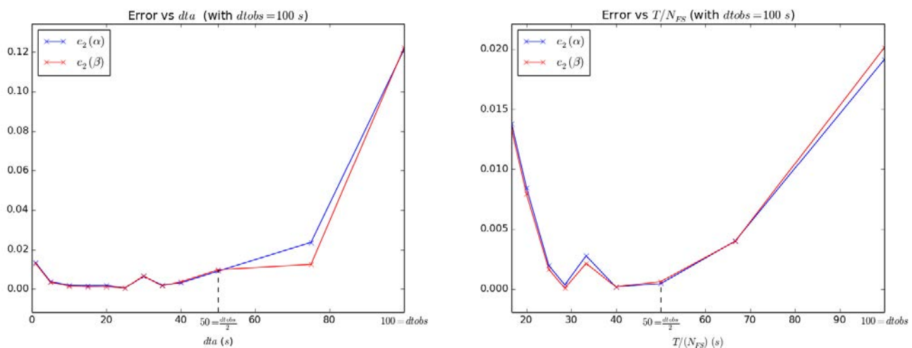
FIGURE 4.3. Roughness identification in the academic test case: errors e_2 on the coefficients (\alpha, \beta) . (Left) IDbasic case: errors vs dt_a . (Right) IDFourier case: errors vs T/N_{FS} .
