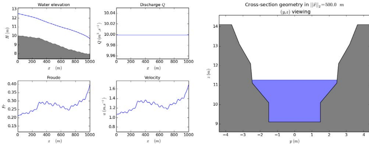
FIGURE 2.2. Academic test case. (Left) Steady state flow for Q_{in} = 10 m^3 \cdot s^{-1} (quite a low value with respect to the considered hydrograph in the forthcoming experiments): (Left, top) Water elevation H (Right, top) Discharge Q . (Left, Bottom) Froude F and (Right, Bottom) Velocity U vs river curvilinear abscissa. (Right) Cross-section example (for x = 500 m).
