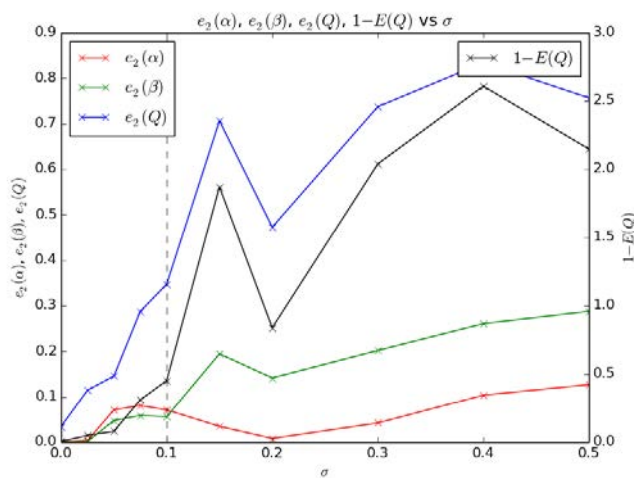
FIGURE 4.5. Error on the identified quantities with \mathbf{k} = (a_0, a_1, b_1, \dots, a_{NFS}, b_{NFS}, \alpha, \beta)^T vs the observation error \sigma (standard deviation of the Gaussian noise). The vertical dashed line represents the expected error of the SWOT mission, both in norm 2 and Nash-Sutcliffe criteria.
