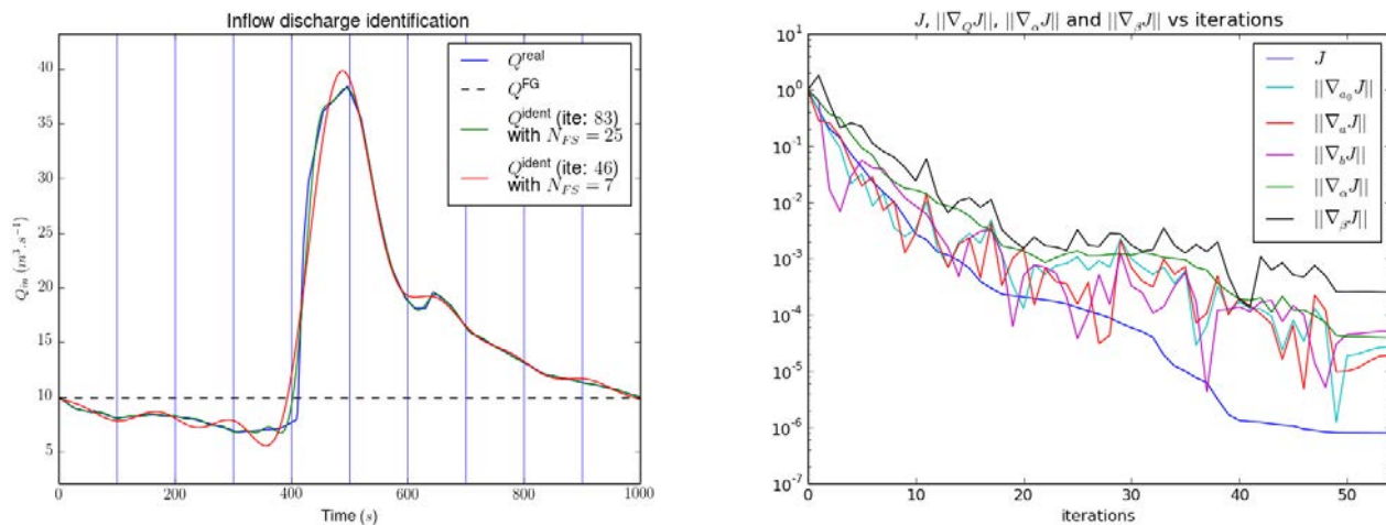
FIGURE 4.2. Discharge and roughness identification in the academic test case (IDFourier case). (Left) Discharge identification with N_{FS} = 7 and N_{FS} = 25 . (Right) Function cost J, \|\nabla_{a_0} J\|, \|\nabla_{a_n} J\|, \|\nabla_\alpha J\| and \|\nabla_\beta J\| vs minimization iterations.
