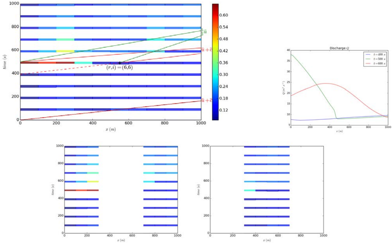
FIGURE 3.2. The identifiability maps in (x, t) in the case: (Top, Left) OD1 (full observations); (Bottom, Left) OD2; (Bottom, Right) OD3.
