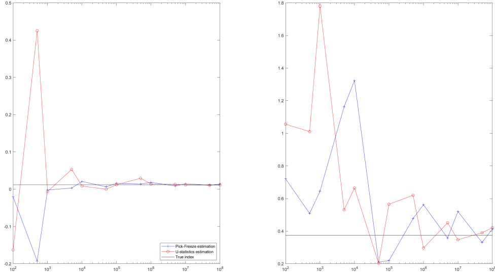
Figure 1: Non-linear model (16). Convergence of both methods when the total number of calls of the computer code increases. The two first order Sobol indices have been represented from left to right. Several total number of calls of the computer code have been considered ranging from n = 100 to n = 10^8 . The x -axis is in logarithmic scale.
