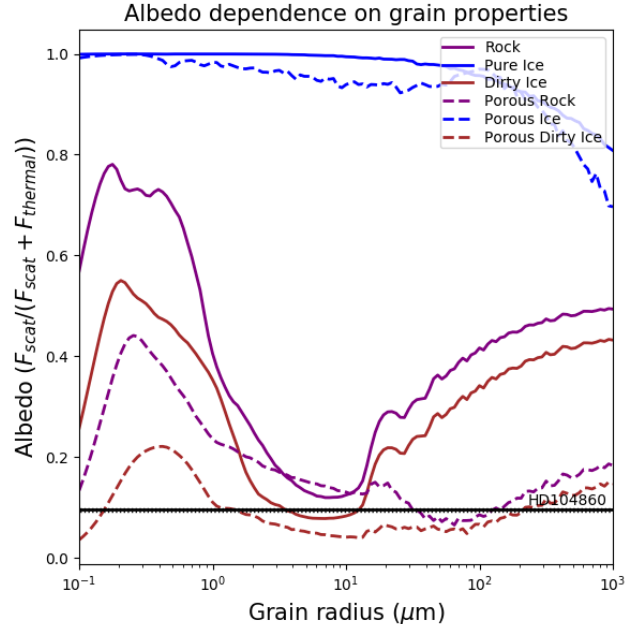
Figure 7. Scattering albedo computed under the Mie theory as a function of grain size for a disk with HD 104860's best fit morphology, assuming different grain compositions: pure ice (blue), dirty ice (red), silicates (purple), and different porosities: compact grains (solid lines) and 90% porous grains (dashed lines). The measured scattering albedo for HD 104860 (black line) rules out water ice compositions and is consistent dirty ice grains larger than \sim 2 \mu\text{m} .
