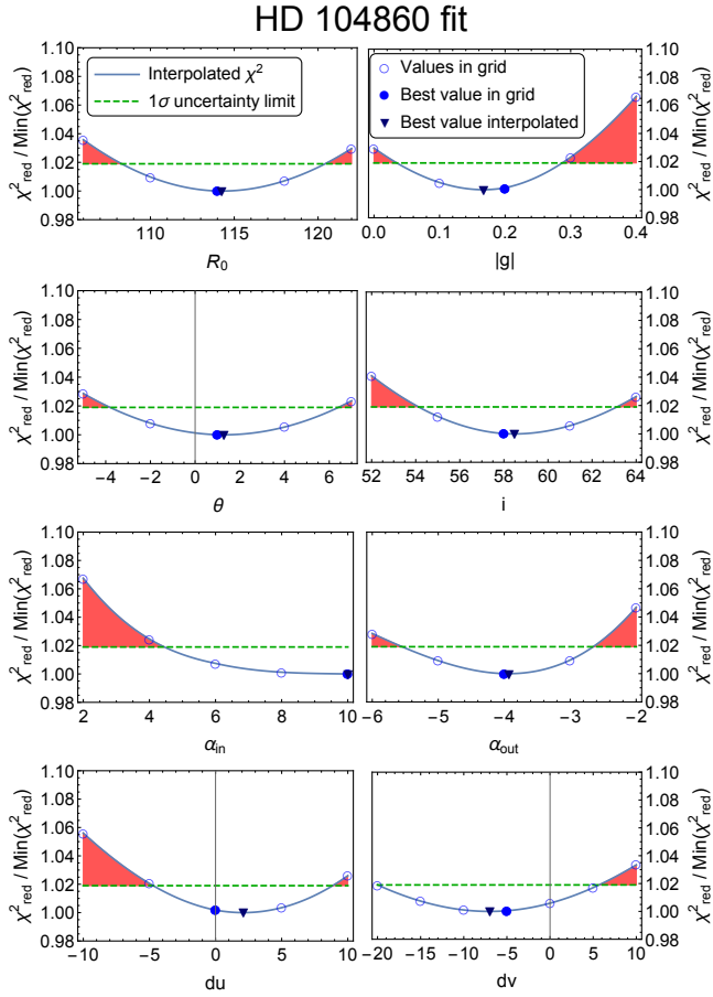
Figure 4. Goodness of fit for each parameter modeling the disk around HD 104860. The chi square values shown for each parameter value in the grid (empty circles) have all the other parameters fixed to their best values in the grid (filled circles). The \chi^2 is interpolated between each parameter value in the grid to refine the best fit values (filled triangles). The dashed green line shows the 1\sigma threshold used to estimate the uncertainties on the parameters, and the red-shaded areas show the parameters values ruled out by our modeling.
