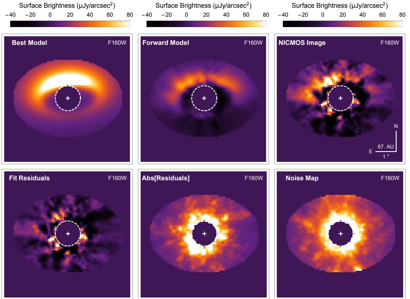
Figure 10. Same as Fig. 5 for HD 192758 in the F160W filter.
