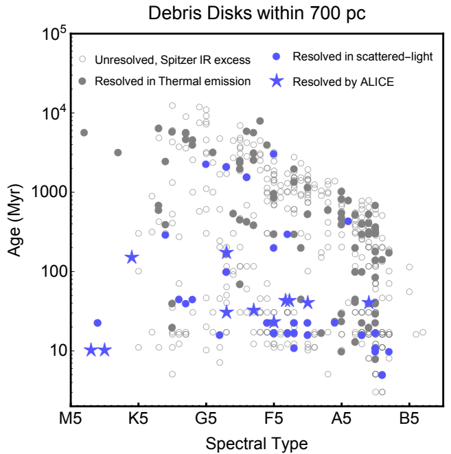
Figure 1. Age and spectral type distribution of the 500 stars within 700 pc with a debris disk detected in thermal emission by the Spitzer Space telescope (grey empty circles Chen et al. 2014), and/or that have been resolved in thermal emission (grey filled circles, 97 systems) or in scattered-light (blue markers, 41 systems). The blue stars highlight the debris disks firstly imaged by ALICE in scattered-light. We note that the Spitzer sample is composed at 94% of stars within 250 pc, with only a few systems beyond 500 pc.
