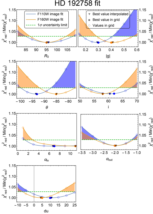
Figure 8. Goodness of fit for each parameter for the disk around HD 192758, in blue for the F110W filter dataset, and in orange for the F160W dataset. The chi square values shown for each value in the grid (empty circles) have all the other parameters fixed to their best values in the grid (filled circles). The \chi^2 is interpolated between each parameter value in the grid to refine the best fit values (filled triangles). The dashed green line shows the 1\sigma threshold used to estimate the uncertainties. The shaded areas show the parameters values ruled out by our modeling.
