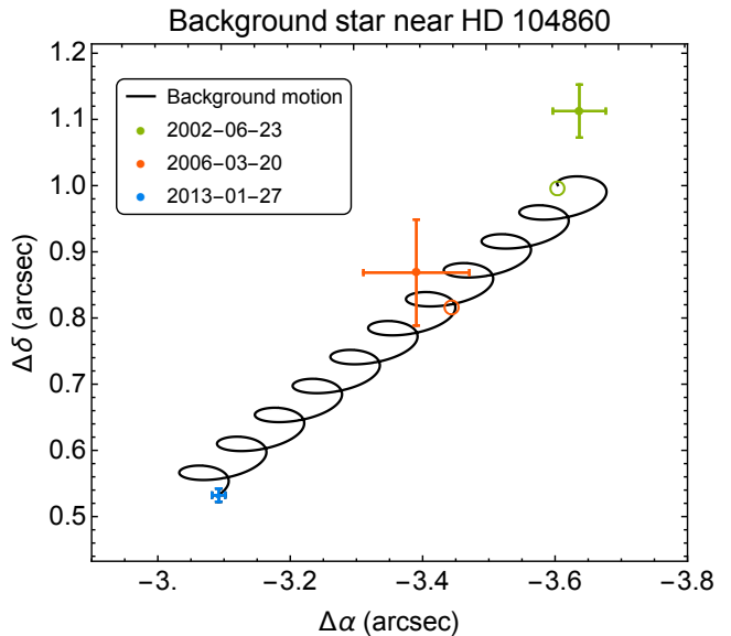
Figure 3. Astrometry of the point source relative to HD 104860, measured with Palomar-P1640 on 2002-06-23 (green) from Metchev & Hillenbrand (2009) , HST-NICMOS on 2006-03-20 (orange), and Keck-NIRC2 on 2013-01-27 (blue). The black line shows the relative motion of a fixed background object from the point source position at epoch 2013-01-27. The empty circles indicate the predicted background position at the corresponding epoch. The point source measured astrometry follows the background track and is not co-moving with HD 104860.
