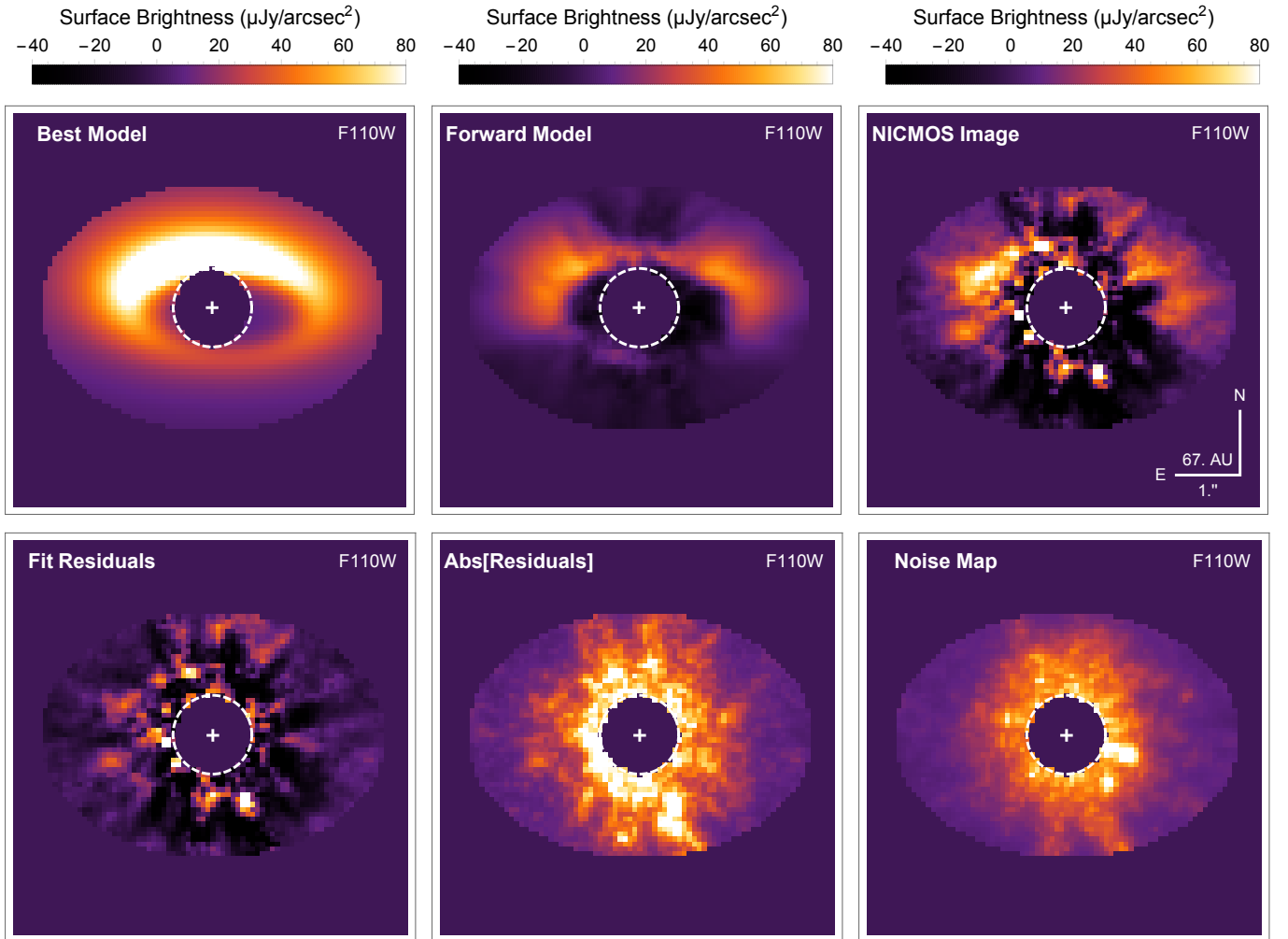
Figure 9. Same as Fig. 5 for HD 192758 in the F110W filter.
