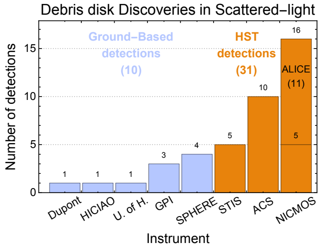
Figure 12. Number of debris disks imaged for the first time in scattered-light per instrument. The ground-based instruments are highlighted in blue (total of 10 discoveries to date) and the HST instruments are highlighted in orange (31 discoveries to date). The NICMOS detections are split between pre-ALICE disks (5 detections) and ALICE disks (11 detections).
