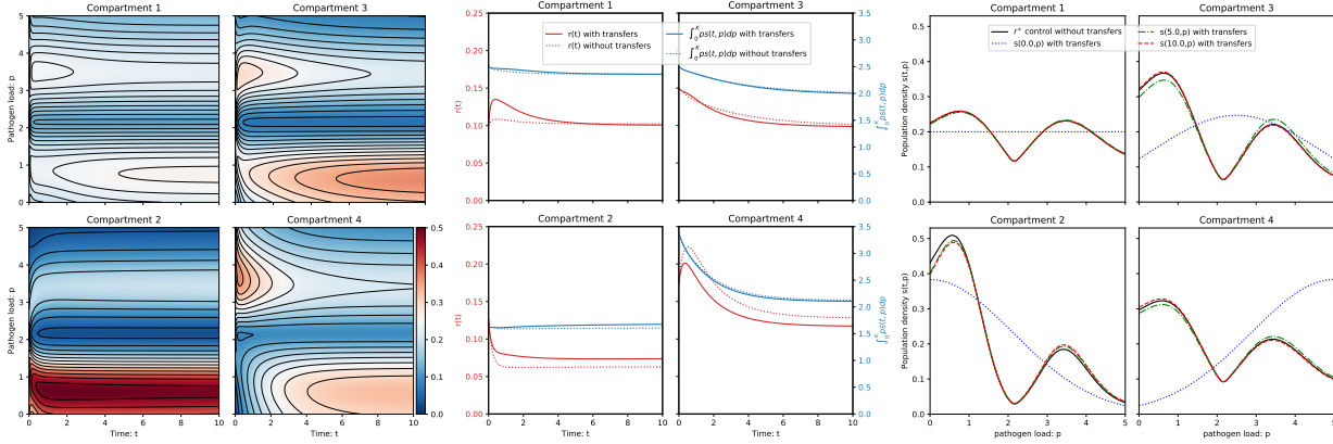
(A) Evolution of the population density s together with level sets in the 4 compartments. (B) Evolution of the reservoir variable r and total pathogen load within the population in the 4 compartments. (C) Population density s at different times in the 4 compartments
