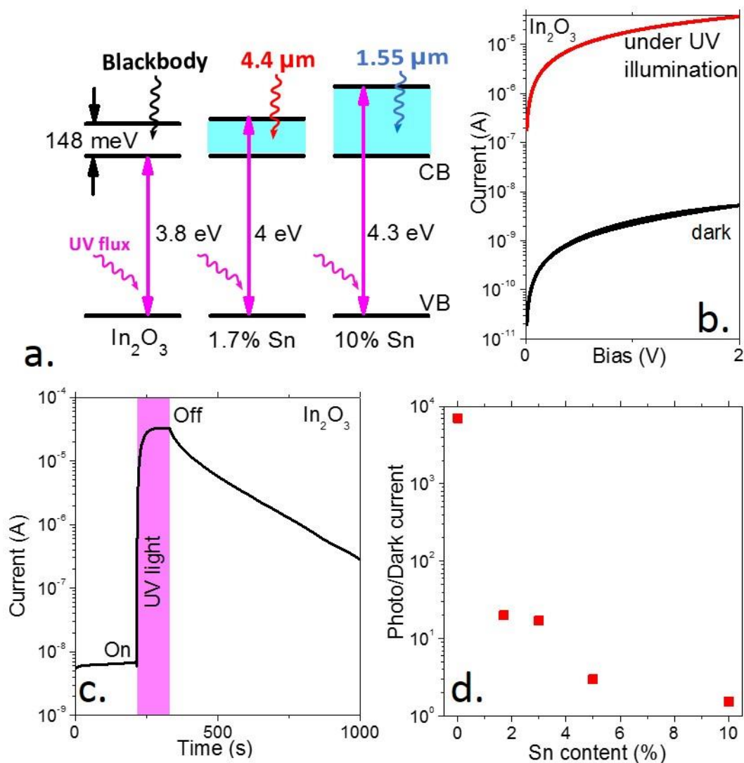
Figure 3a. Band diagram of undoped, 1.7% Sn and 10% Sn doped ITO nanocrystals. For all materials, the bottom of the conduction band and the top of the valence band are treated as identical to the undoped material. The energy of the first empty state of the conduction band is determined using a Tauc plot, see figure S3. b. I-V curve of \text{In}_2\text{O}_3 nanoparticles under dark condition and under UV illumination. c. Current as a function of time while a thin film \text{In}_2\text{O}_3
