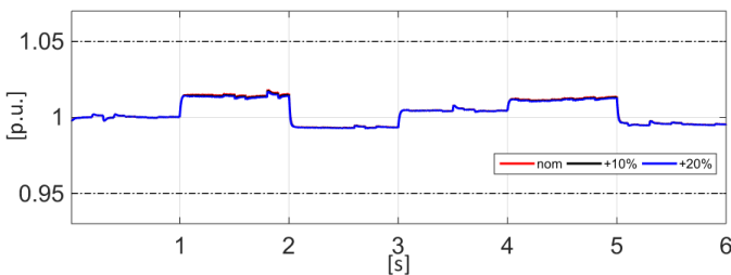
Fig. 11. The DC grid voltage V_{dc} with the parameters errors.
